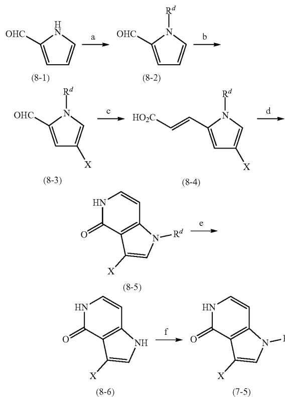
(Scheme 8)
