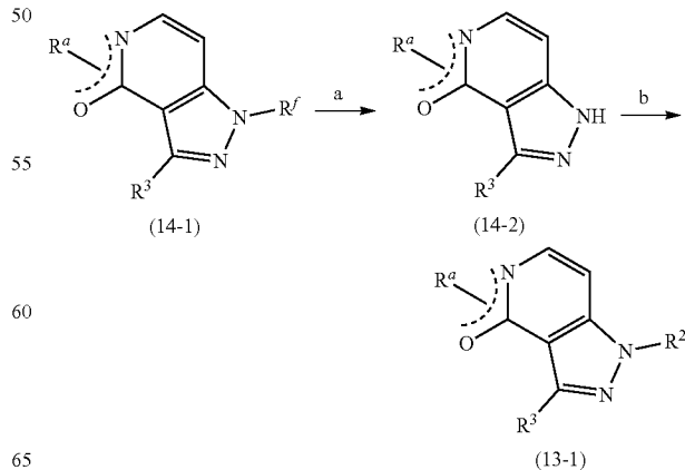
(Scheme 14)
