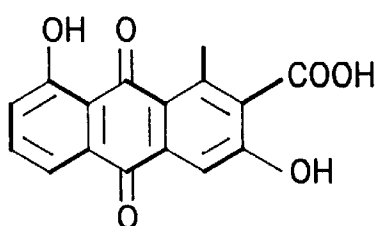
DMAC (28) (minPKS, KR, ARO, CYC; all act )
