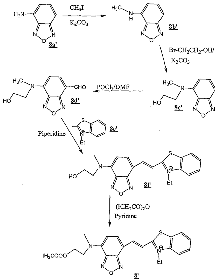
Scheme VIIa
