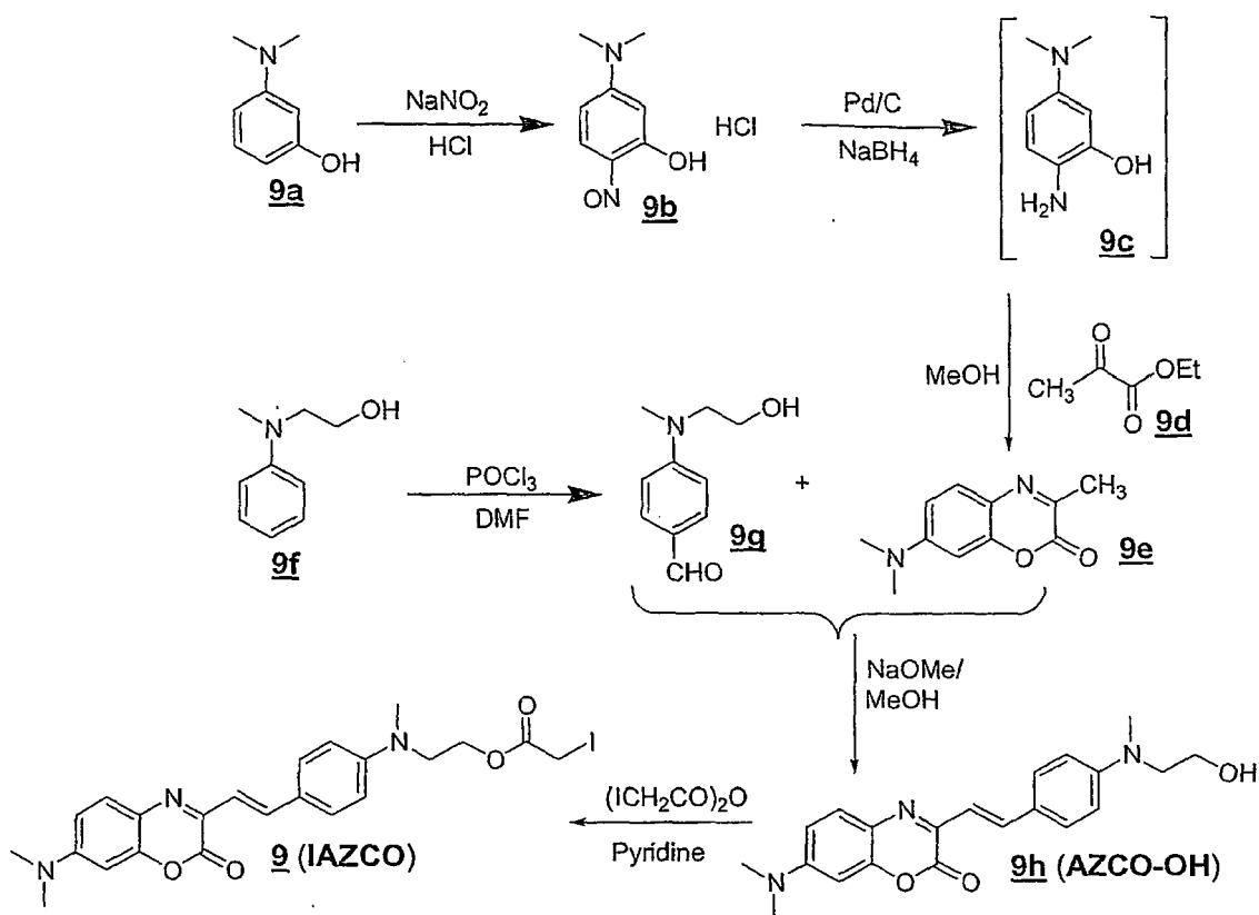
Scheme VIII
