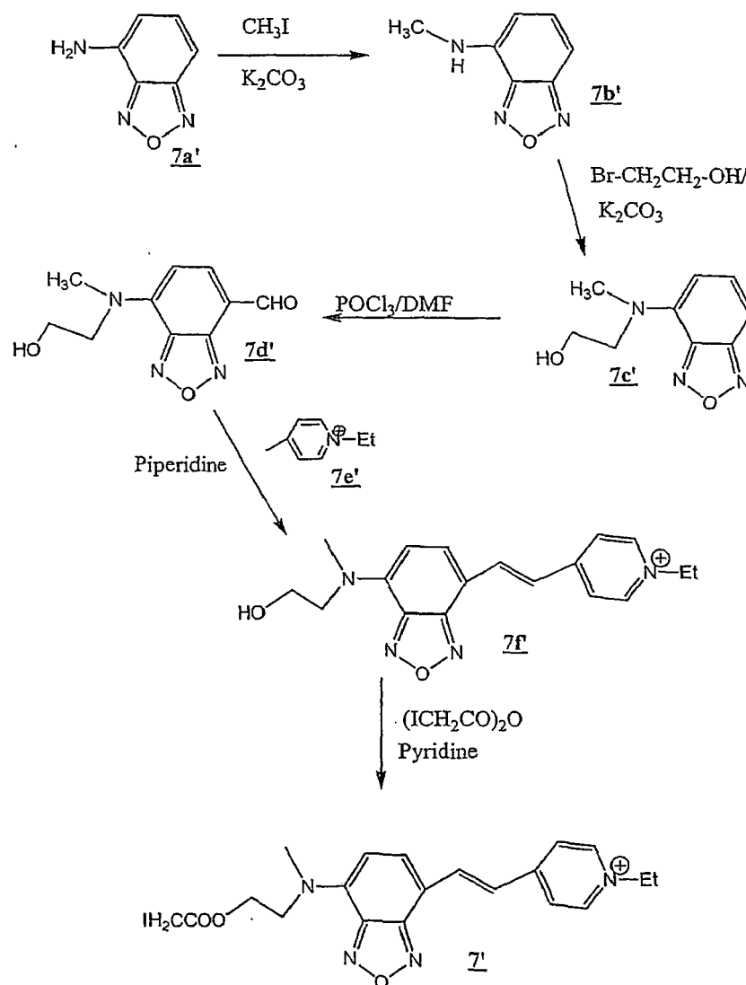
Scheme VIa
