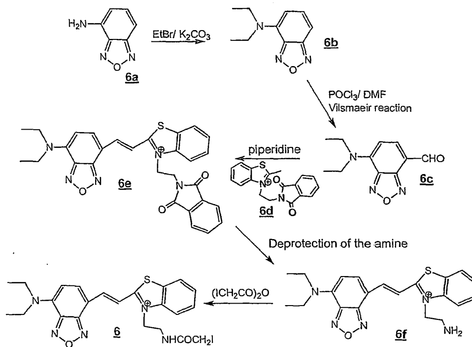
Scheme V
