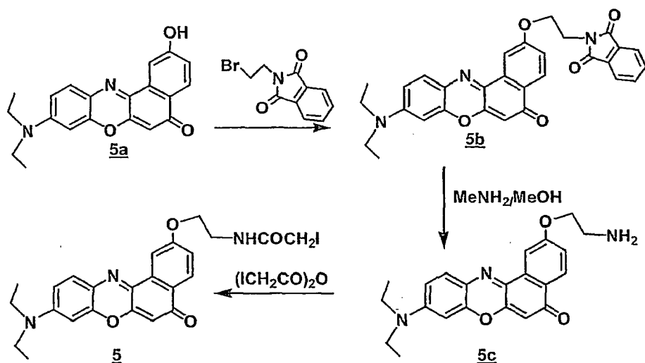
Scheme IV
