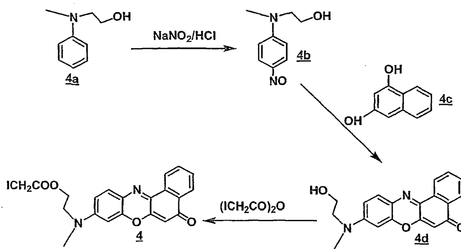
Scheme III
