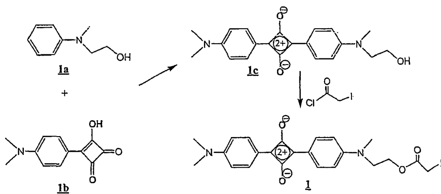
Scheme I
