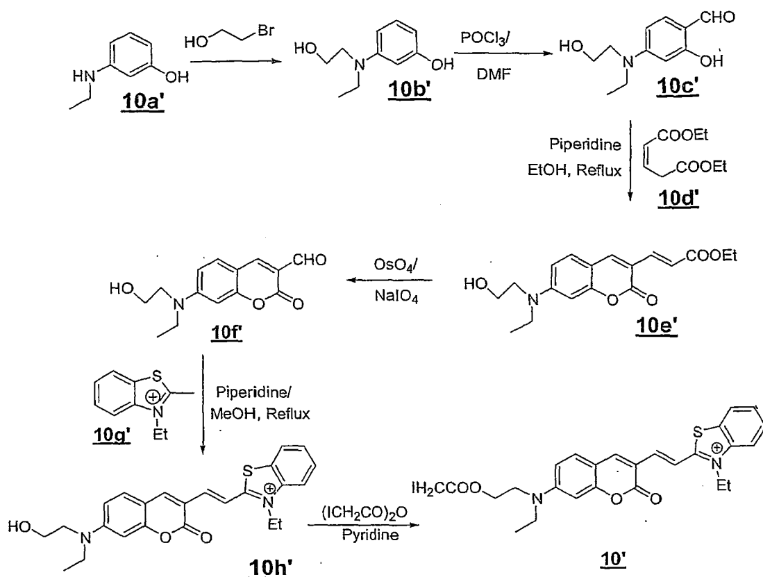
Scheme IXa
