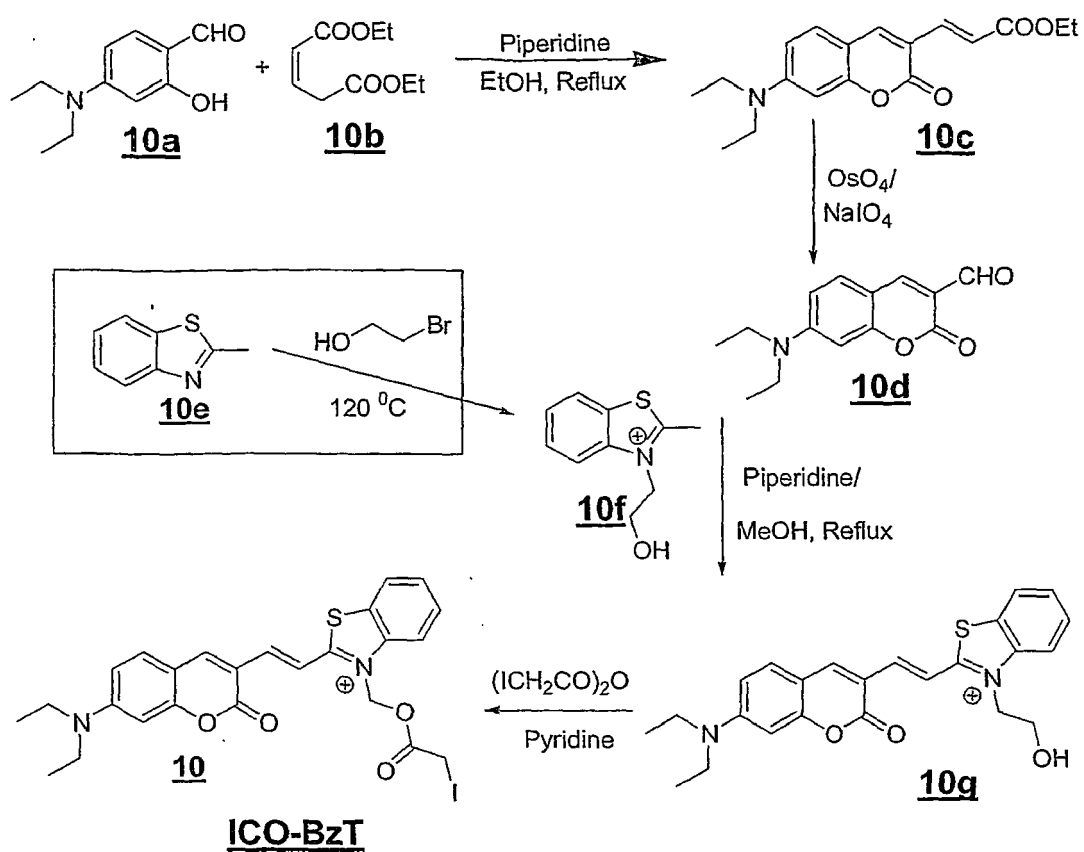
Scheme IX
