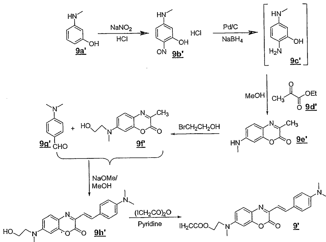
Scheme VIIIa
