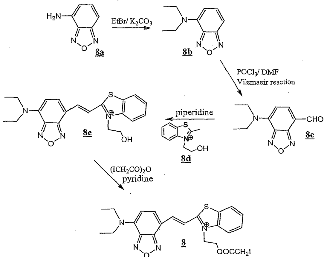
Scheme VII
