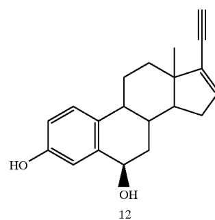
Scheme 4. 17-Ethylenation of ketones
