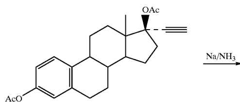
Scheme 3. Further syntheses of norpregnanes
