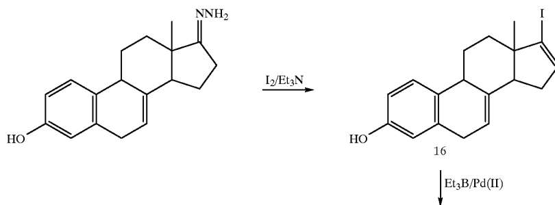
Scheme 5. Pd(II)-catalyzed synthesis of 19-norpregnanes.
