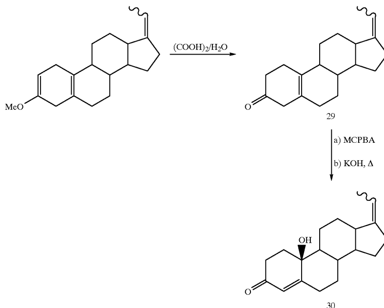
Scheme 8. Synthesis of 19-norpregnanes.
