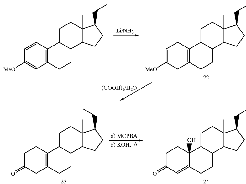
Scheme 6. Synthesis of 19-norpregnanes
