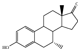
7α-METHYLESTRONE
