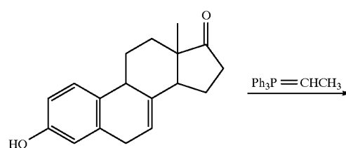
Scheme 4. 17-Ethylenation of ketones
