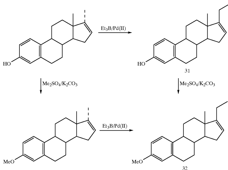
Scheme 9 Synthesis of 19-Norpregna-1,3,5(10), 16-tetraen-3-yl methyl ether
