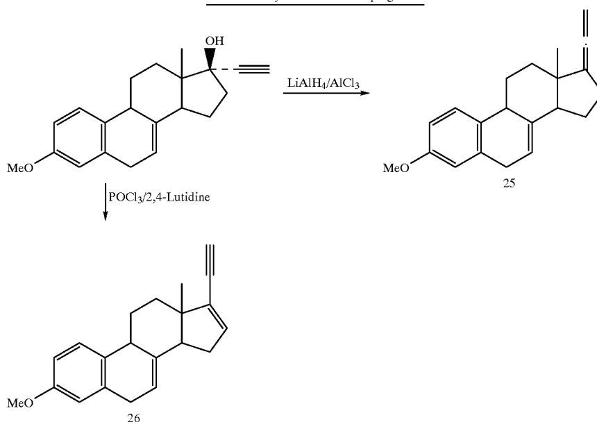
Scheme 7. Additional syntheses of 19-norpregnes.
