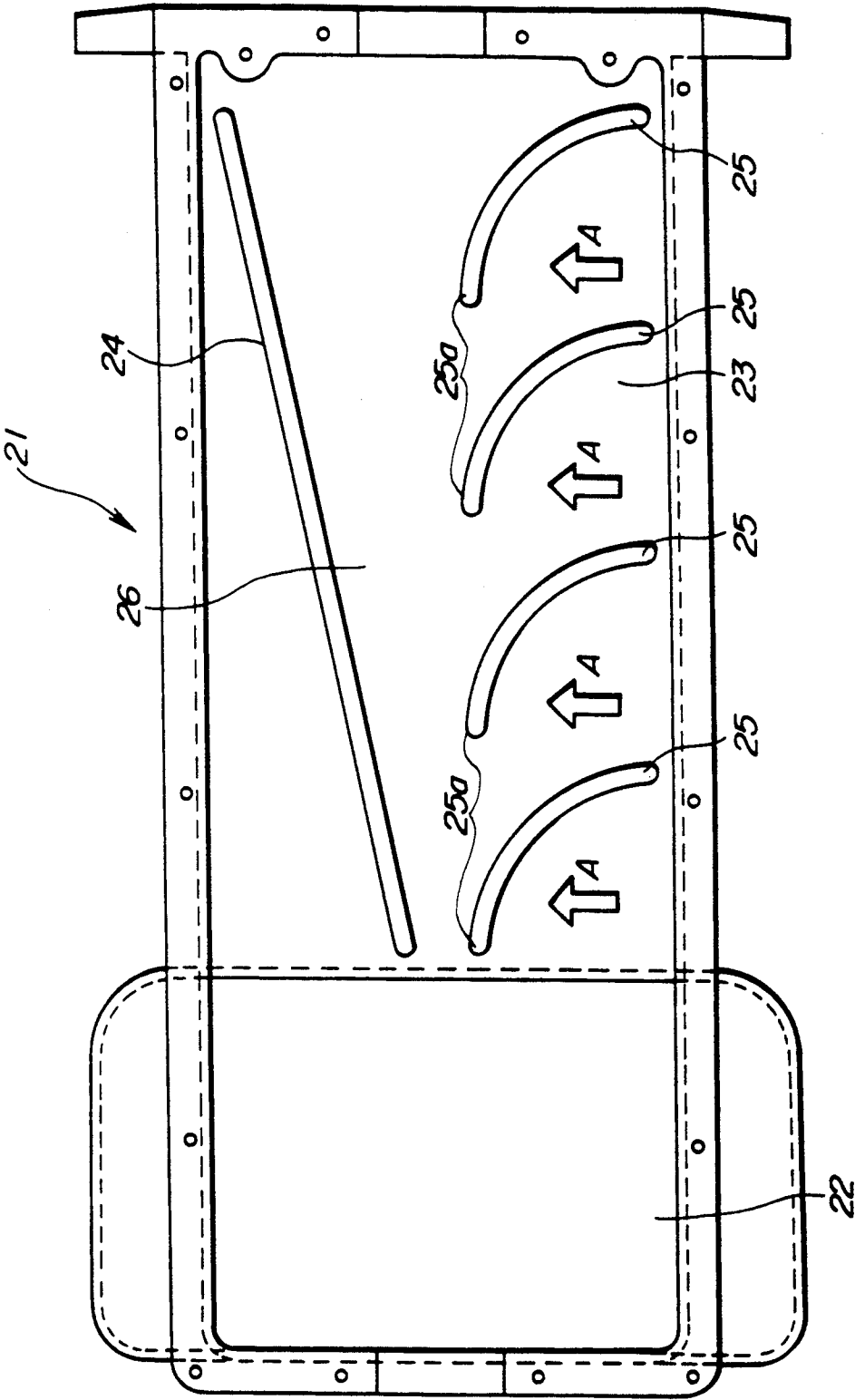
FIG. 6 (PRIOR ART)
