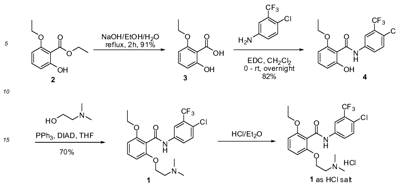
Scheme 1: Synthesis of Compound 1.
