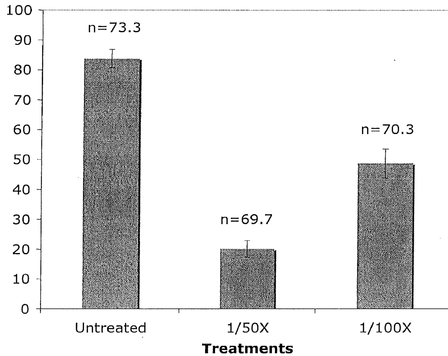
Figure 6: Percentage of lesions with conidia
