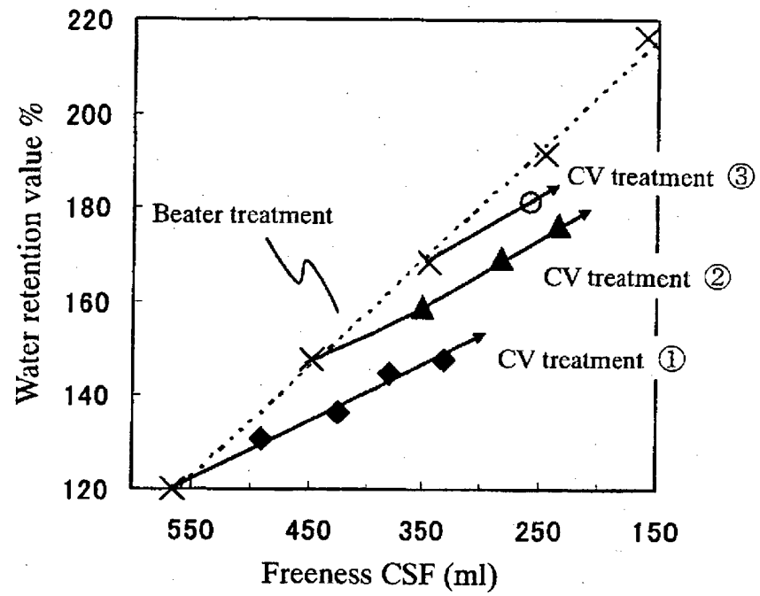
Relationship between freeness and water retention value
