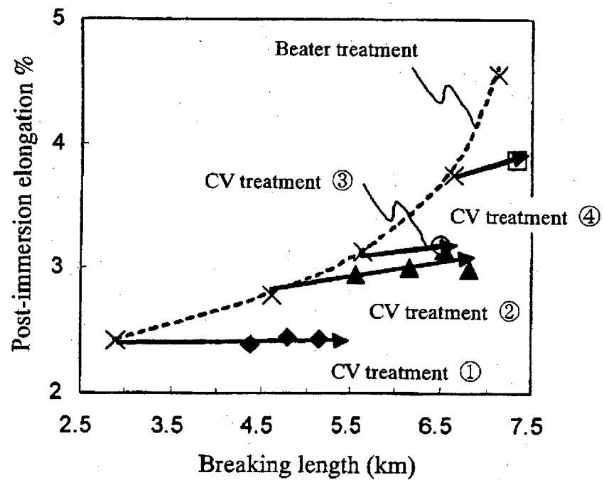
Relationship between breaking length and post-immersion elongation
