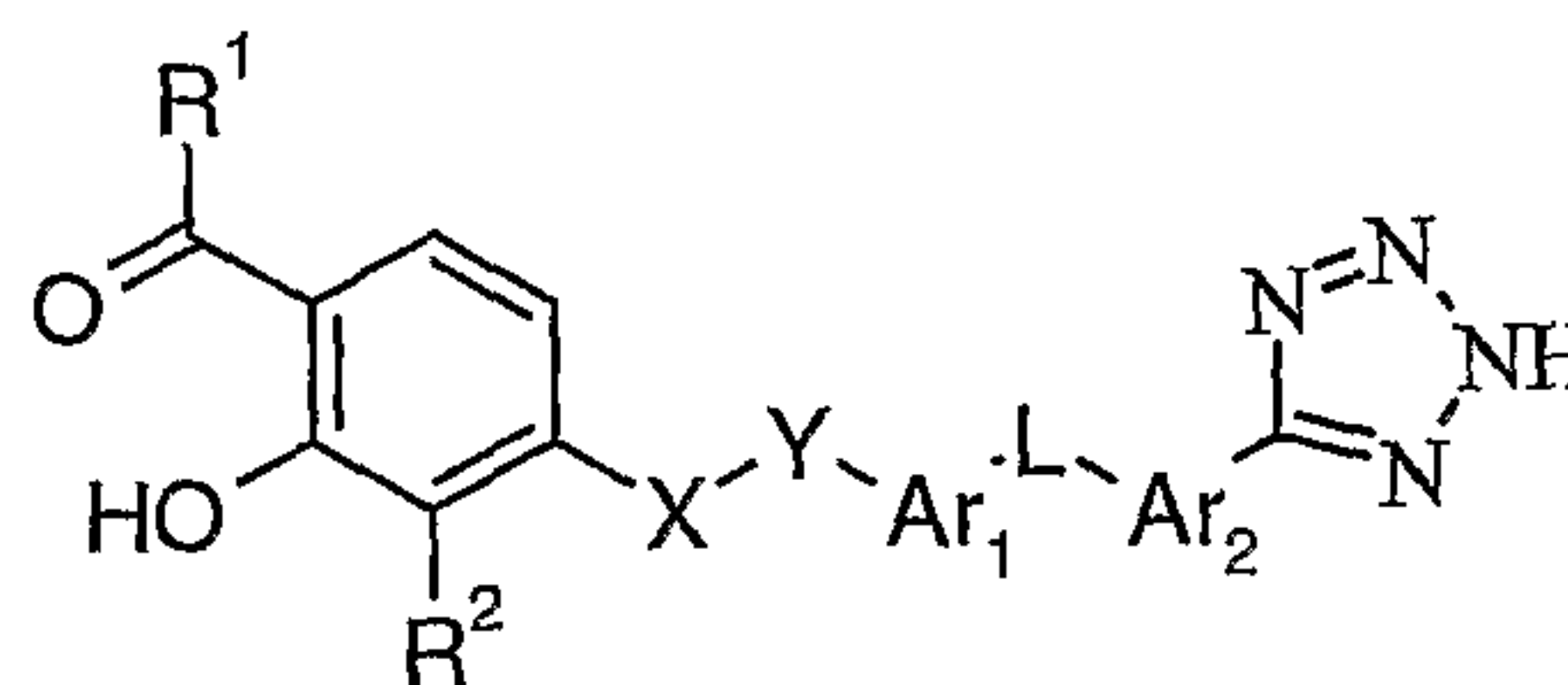
tautomer II
