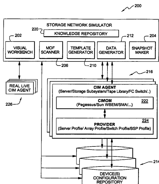
ARCHITECTURE OF STORAGE NETWORK SIMULATOR
