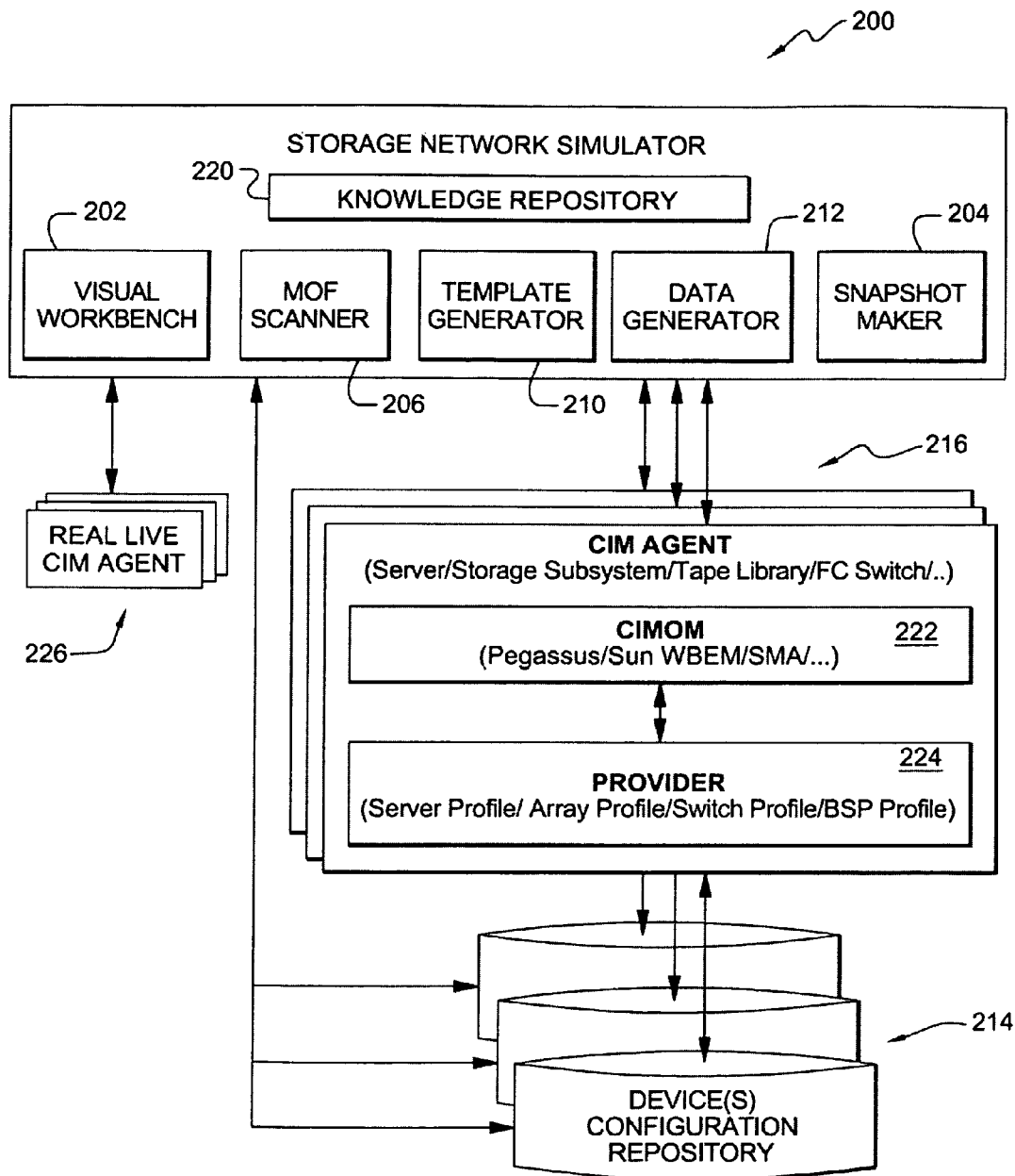
ARCHITECTURE OF STORAGE NETWORK SIMULATOR
