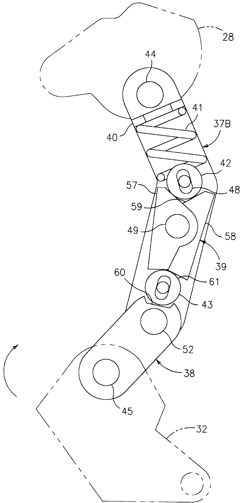
FIG. 4 (CLOSED)
