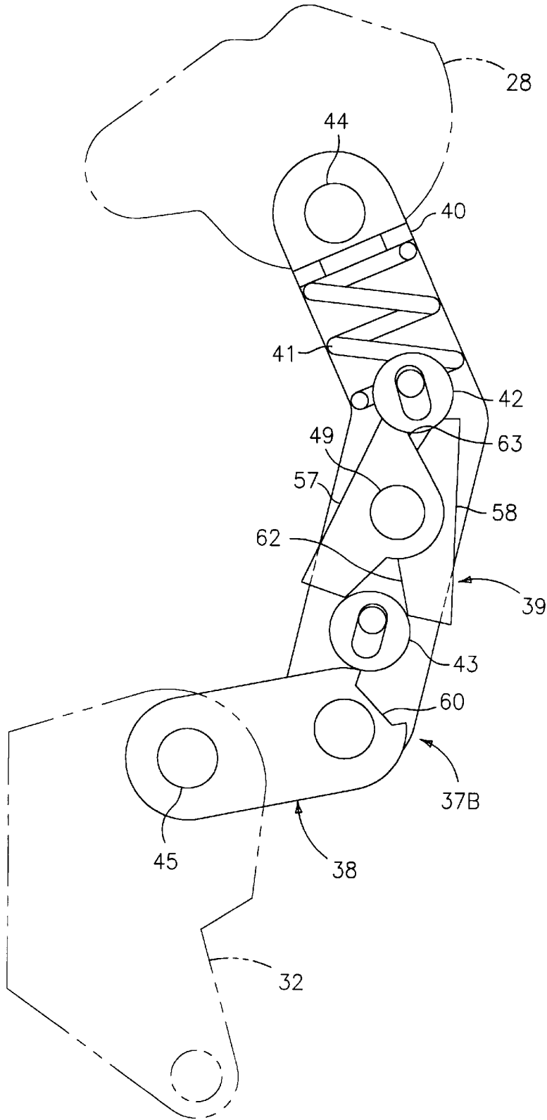
FIG. 5 (TRIPPED)
