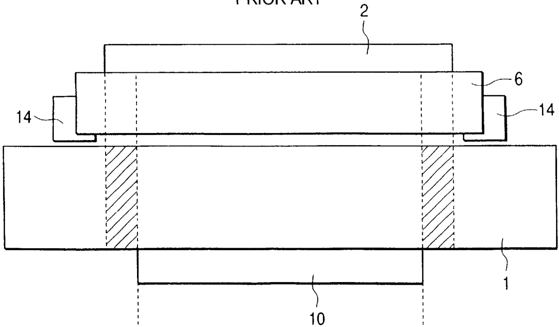
FIG. 7 PRIOR ART
