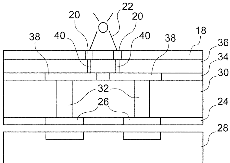
FIG. 2 (PRIOR ART)
