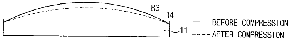
FIG. 6 CONVENTIONAL ART
