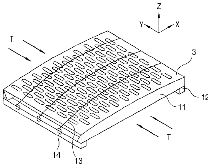
FIG. 7 CONVENTIONAL ART
