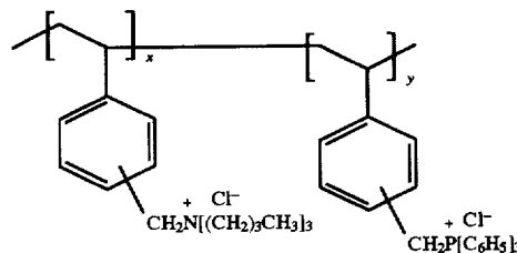
polyvinylbenzyltributyl ammonium chloride-co-polyvinylbenzyltriphenyl phosphonium chloride
