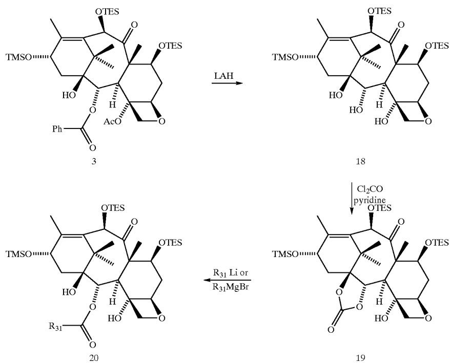
Scheme 6
