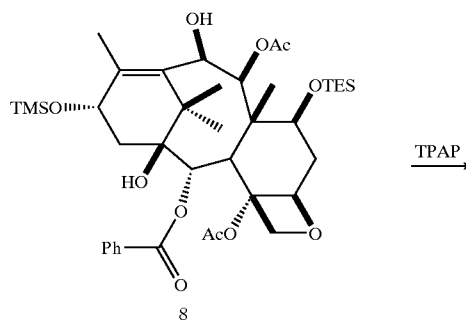
REACTION SCHEME 3
