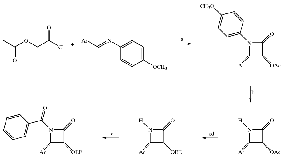
Scheme A
