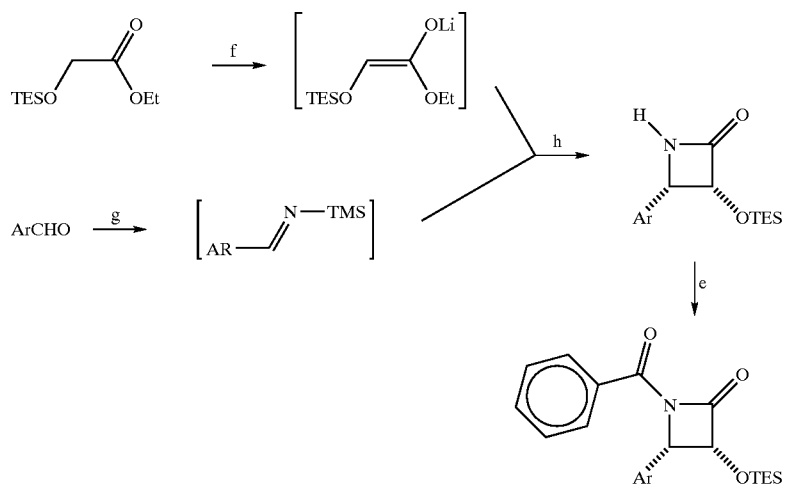
Scheme B
