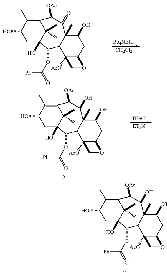
REACTION SCHEME 1
