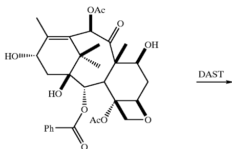
REACTION SCHEME 12
