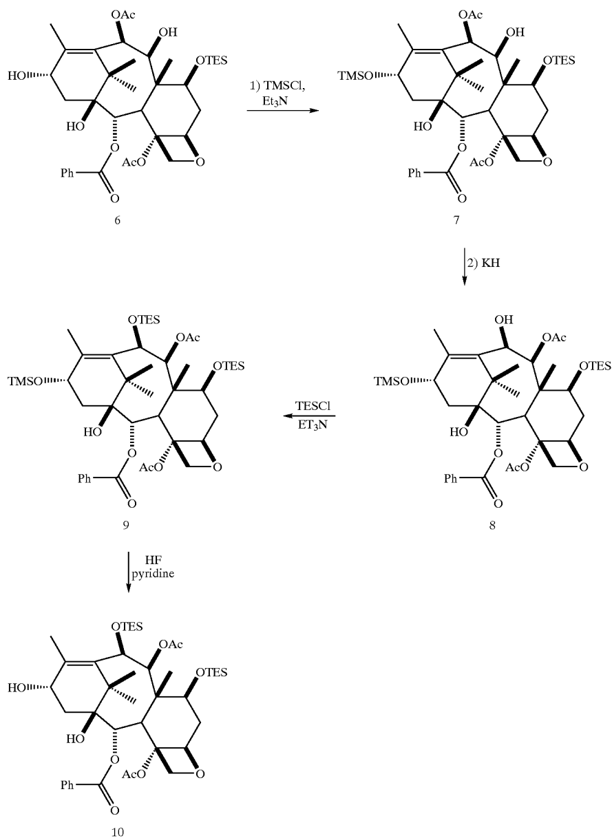
REACTION SCHEME 2
