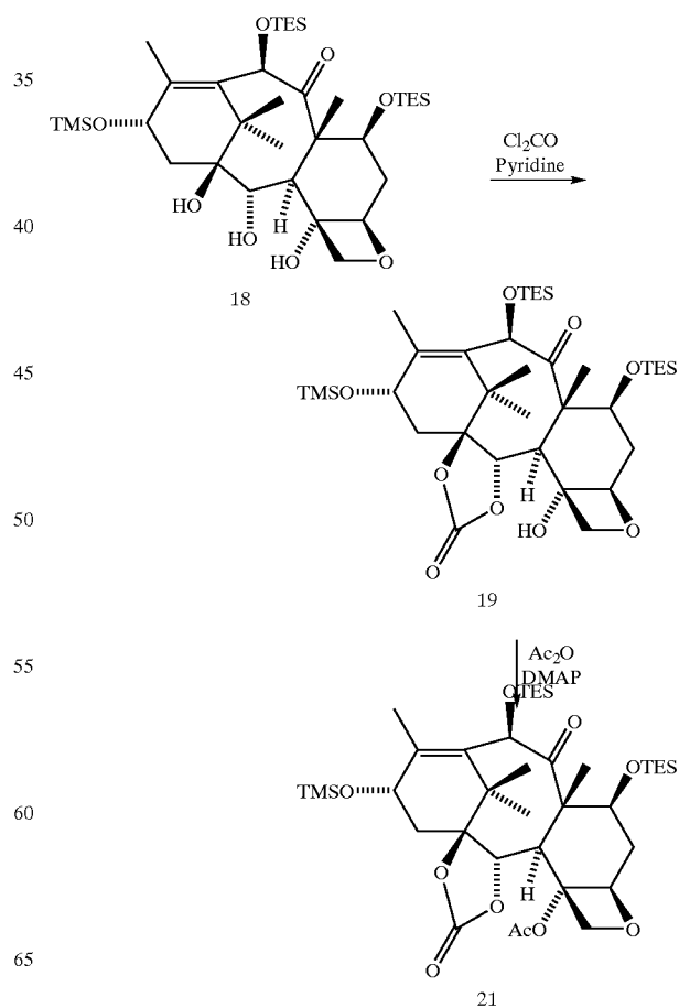
Scheme 8
