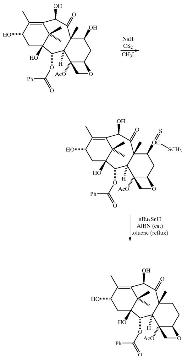
REACTION SCHEME 11
