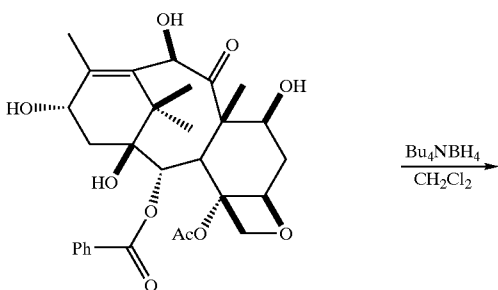
REACTION SCHEME 4
