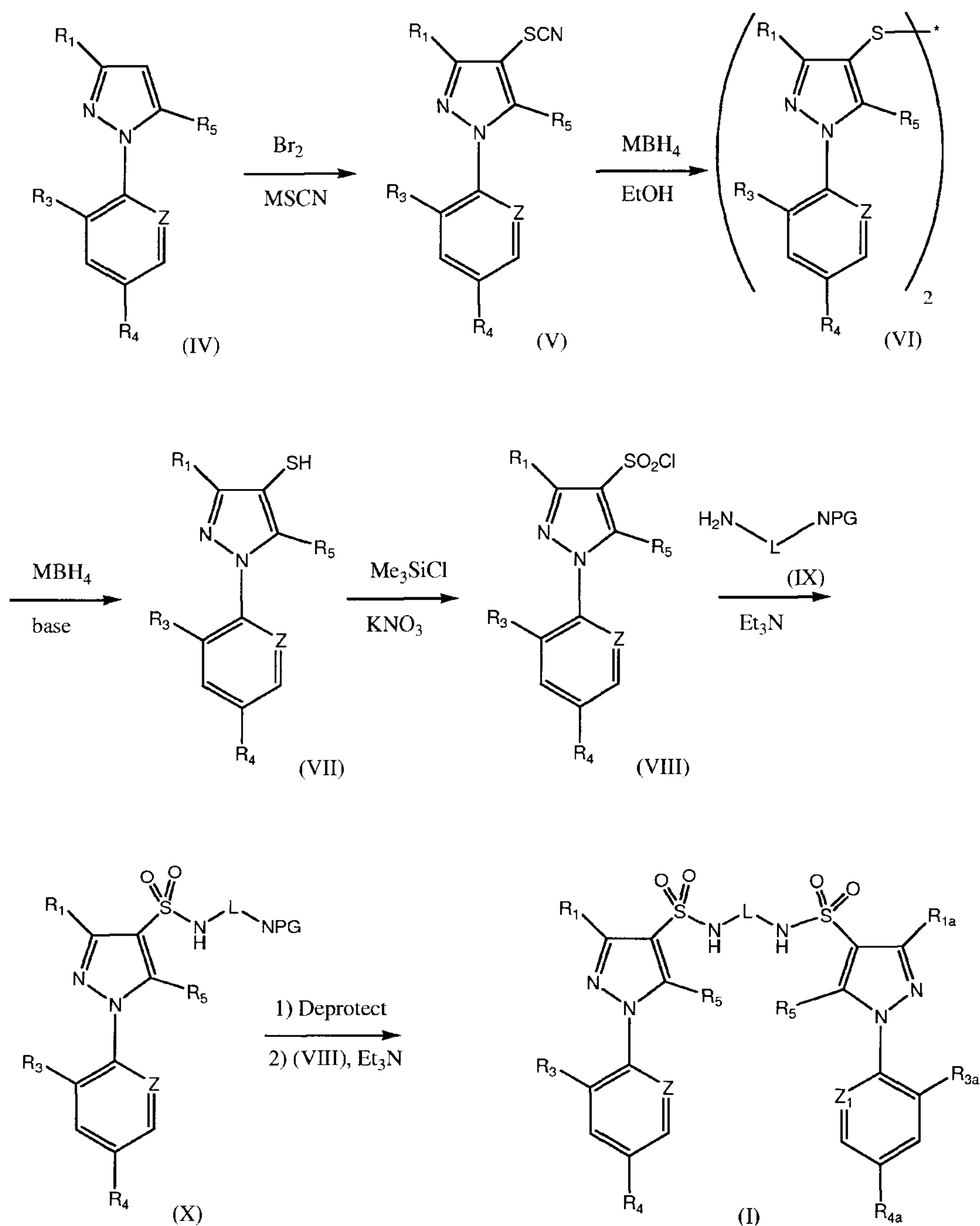
Scheme 1. Synthesis of compounds of formula (I).
