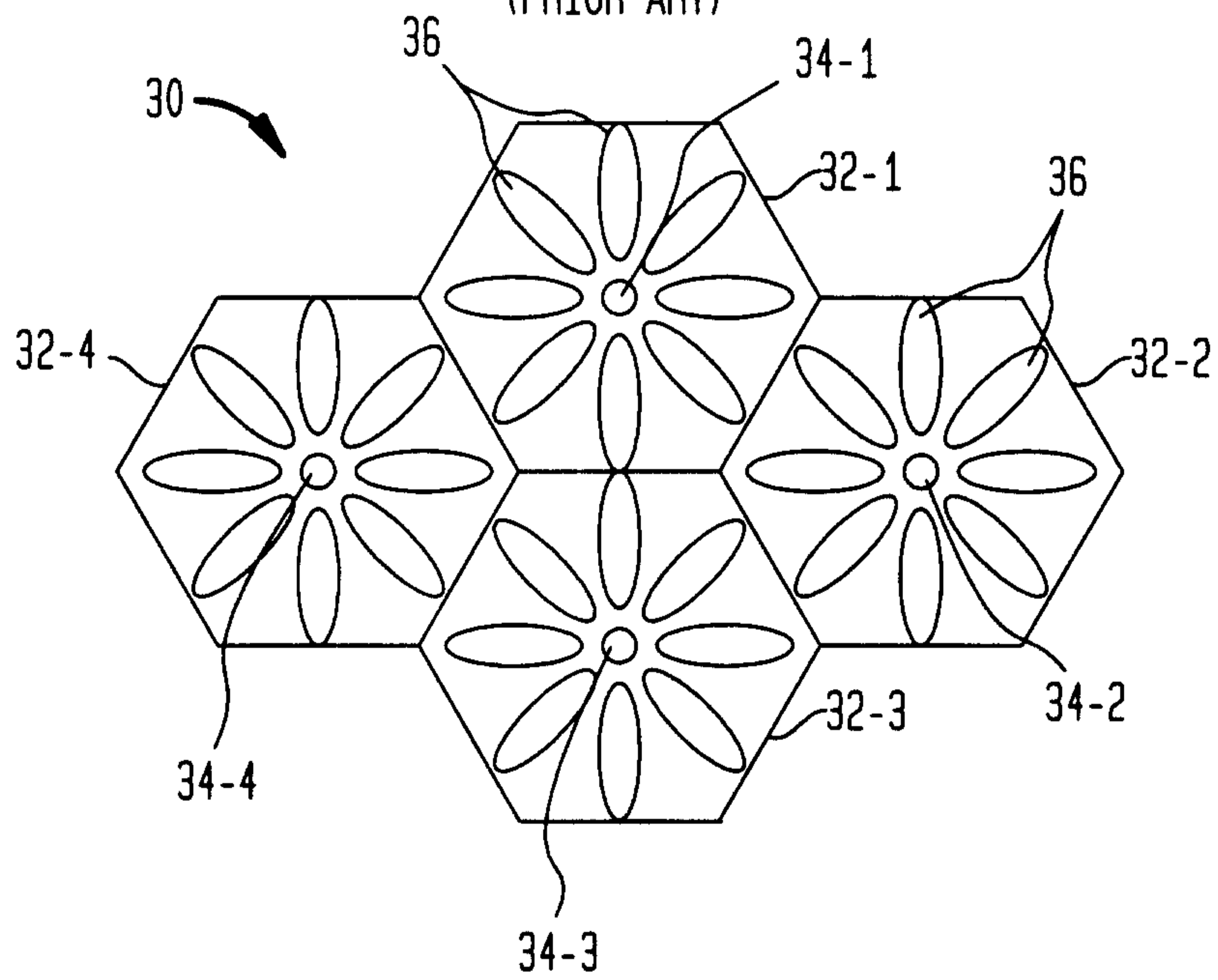
FIG. 3 (PRIOR ART)
