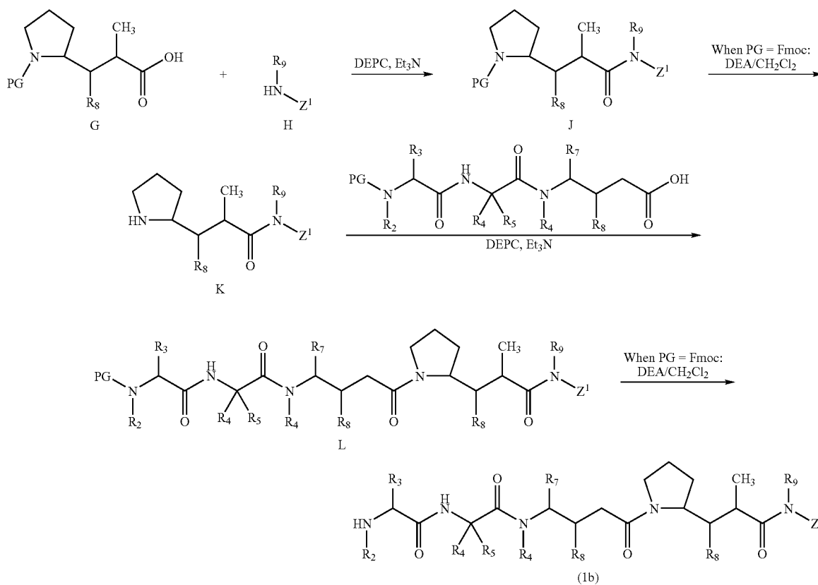
Scheme 6
