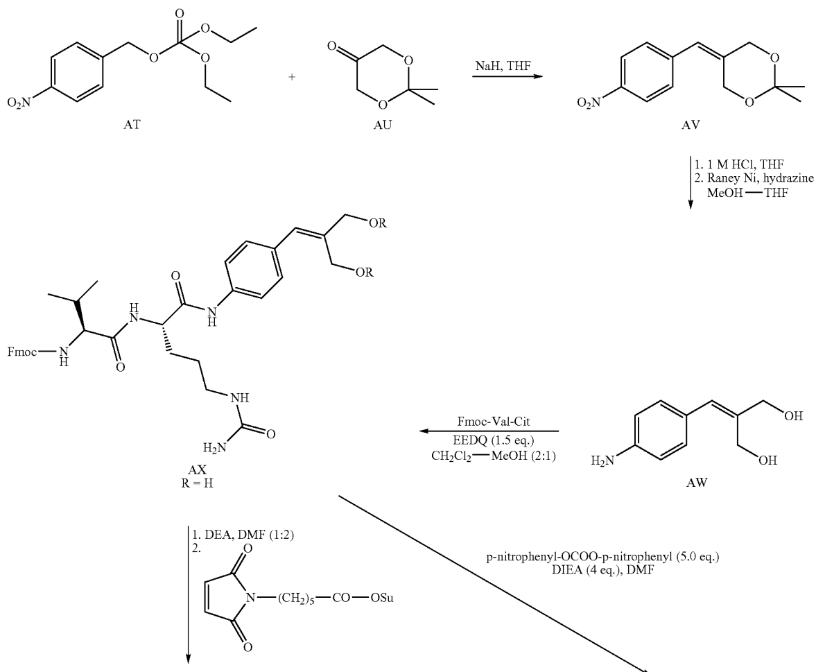
Scheme 15
