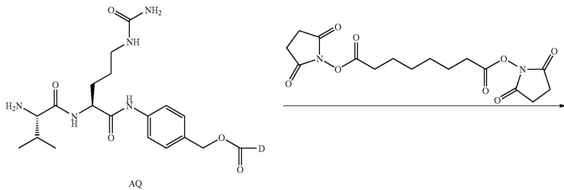
Scheme 14a
