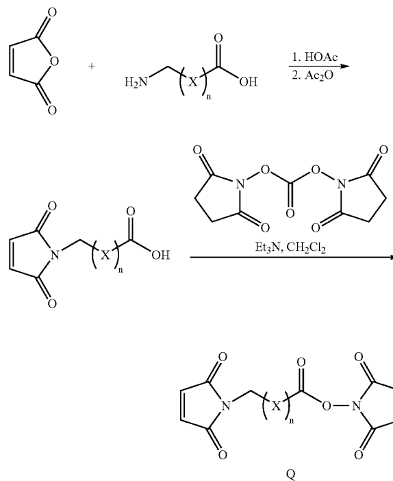
Scheme 8
