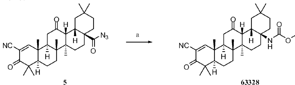
Scheme 16:
