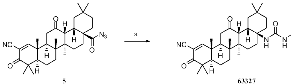
Scheme 15:
