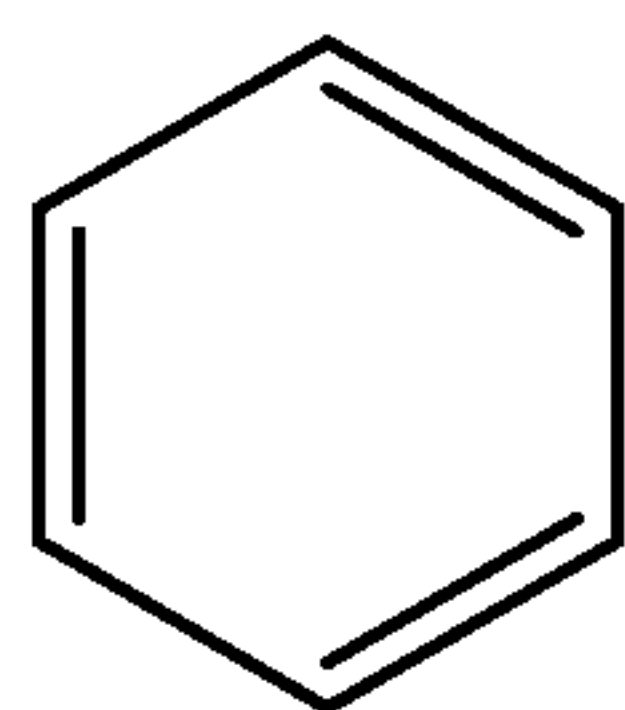
phenyl
