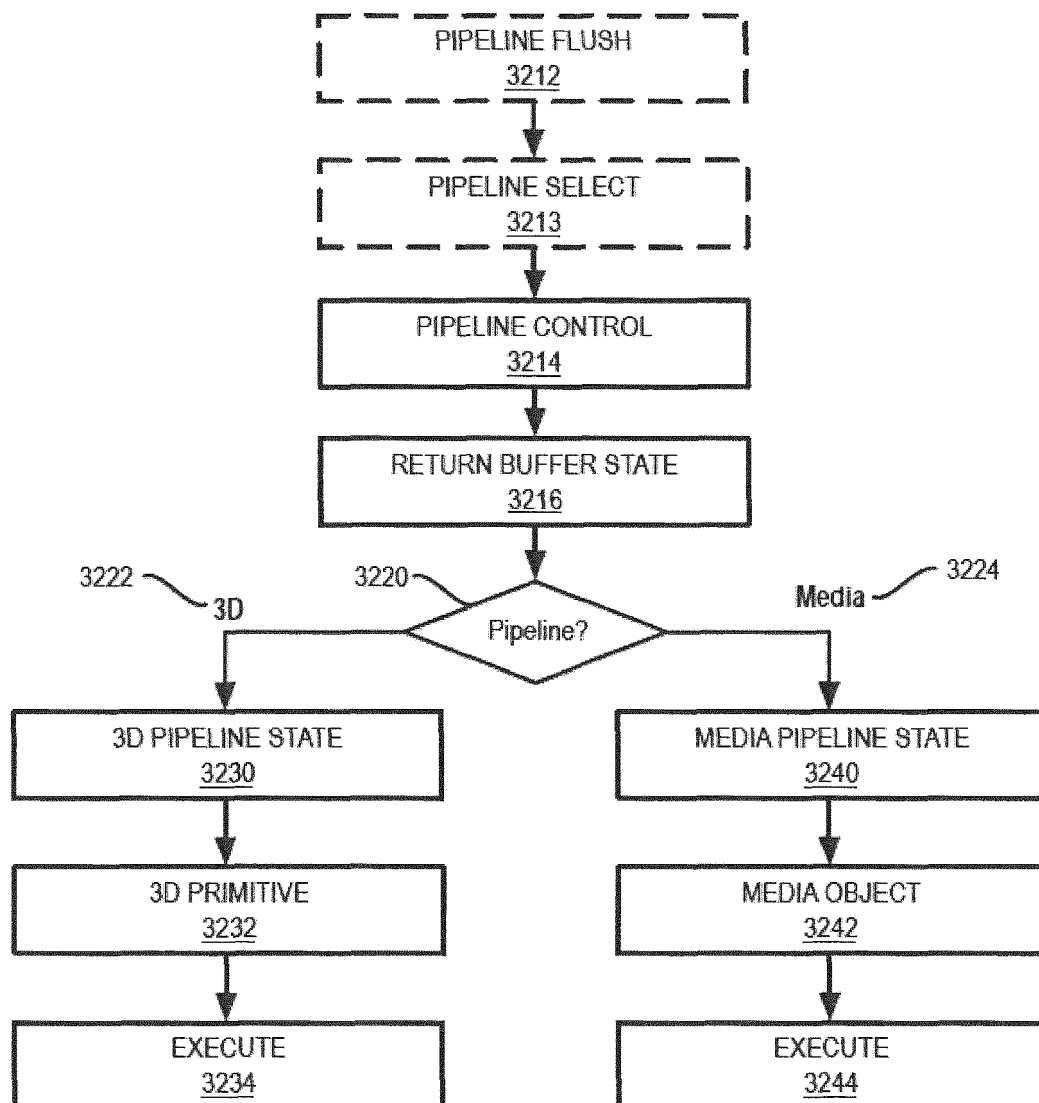
FIG. 32B GRAPHICS PROCESSOR COMMAND SEQUENCE
