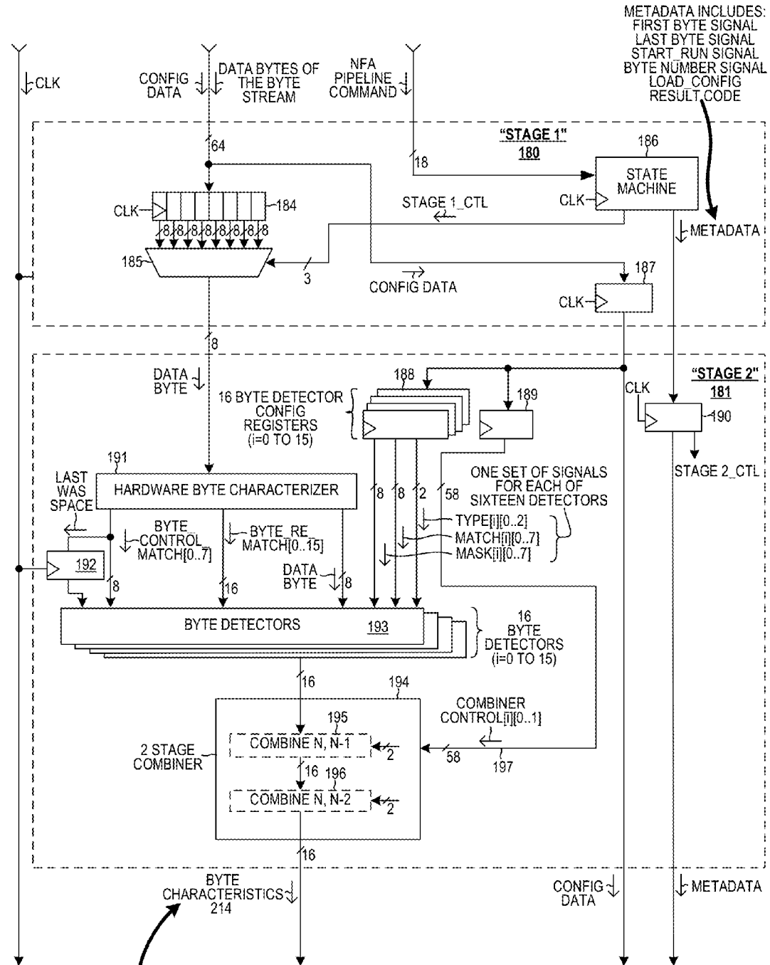
NFA PIPELINE FIG. 12A
