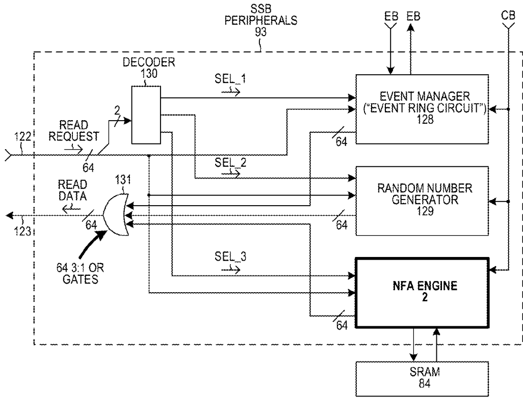
SSB PERIPHERALS BLOCK FIG. 6
