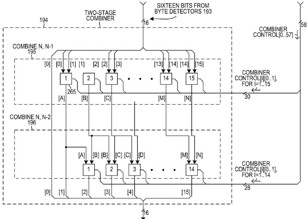
TWO-STAGE COMBINER FIG. 19
