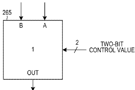
COMBINER CELL FIG. 20
