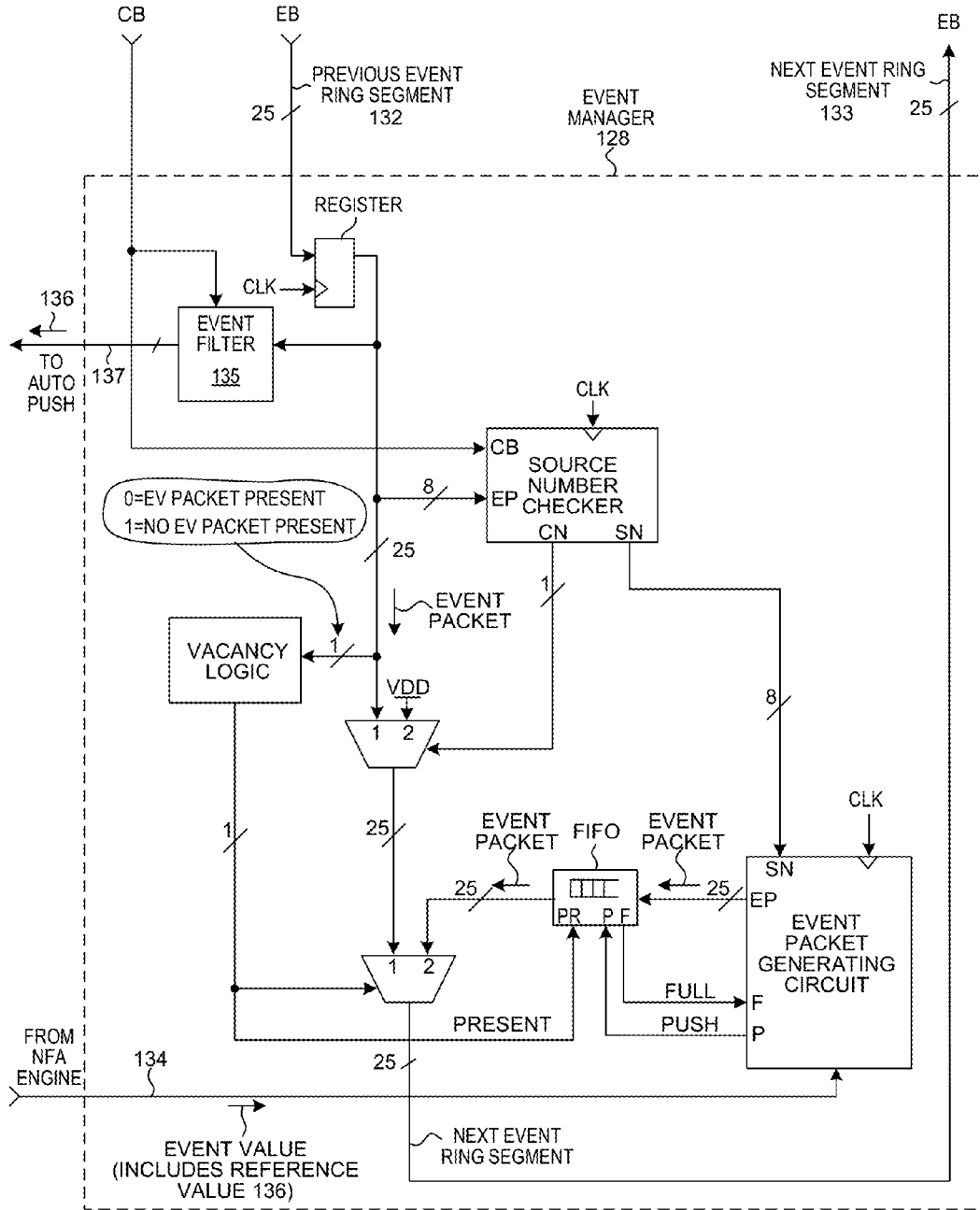
EVENT MANAGER ("EVENT RING CIRCUIT") FIG. 7
