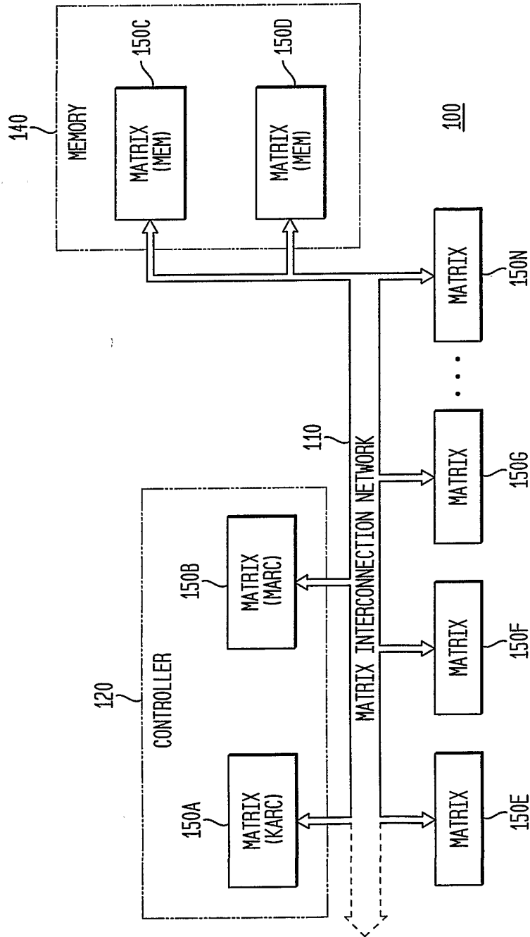
FIG. 4 ADAPTIVE COMPUTING ENGINE (ACE)
