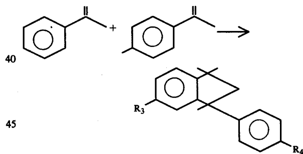
Reaction Scheme #8:
