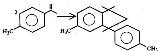
Reaction Scheme #6:
