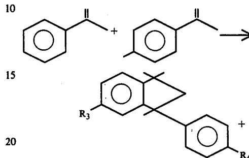
Reaction Scheme #7:
