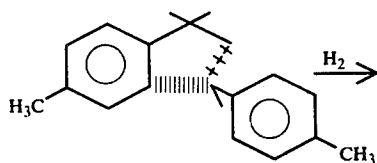
Reaction Scheme #6:
