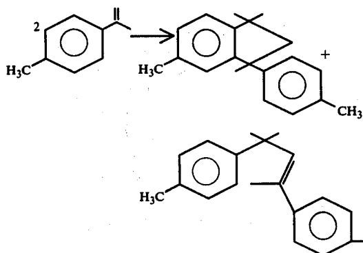
Reaction Scheme #4:
