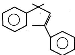
Reaction Scheme #7:
