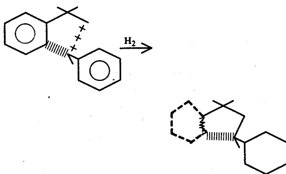
Reaction Scheme #4:
