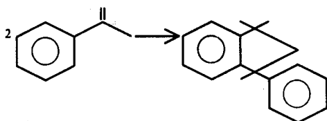
Reaction Scheme #3:
