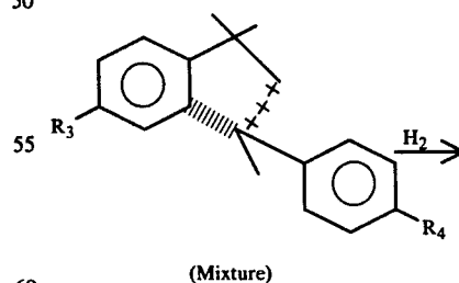
Reaction Scheme #9:
