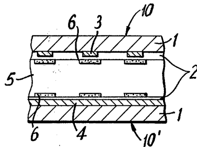
(PRIOR ART) FIG. 1b
