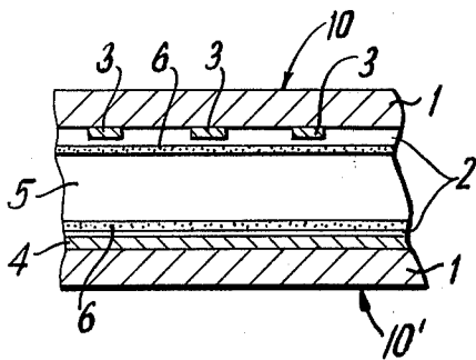
(PRIOR ART) FIG. 1a
