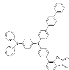
H24
