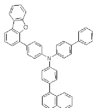
H6
