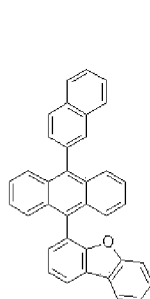
Host 13
