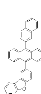
Host 15
