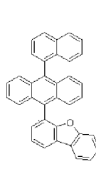
Host 3
