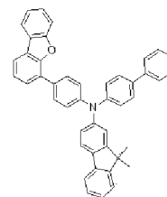
H12
