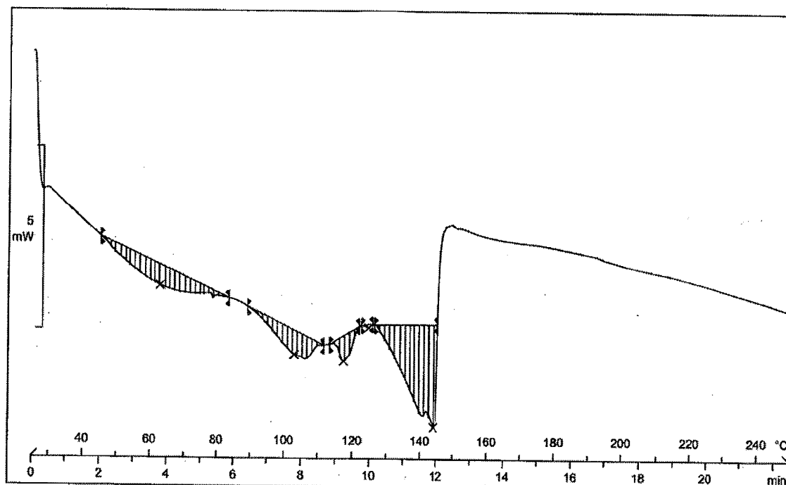
Figure 67: DSC thermogram of Dasatinib form AK
