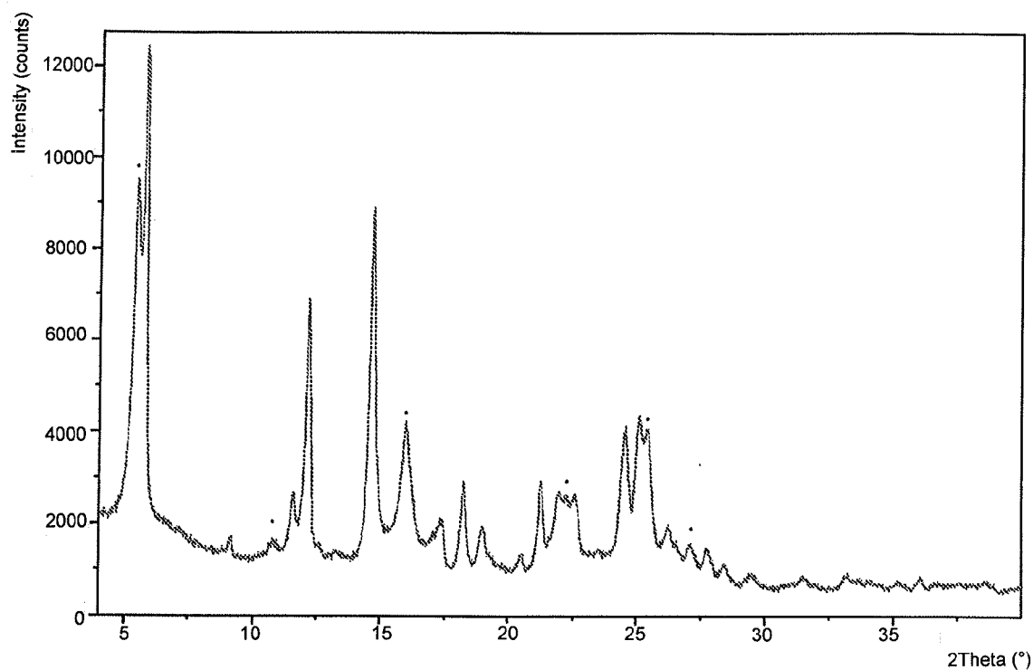
Figure 13: PXRD pattern of Dasatinib mixture of forms G and M
