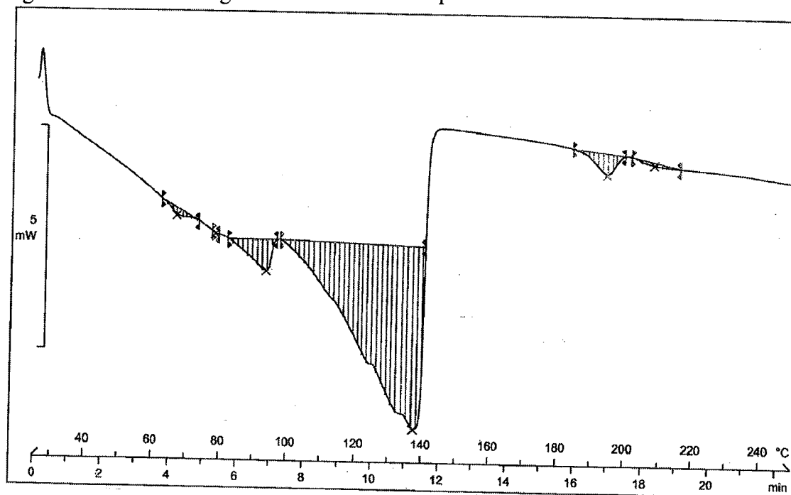
Figure 93: DSC thermogram of Dasatinib amorphous
