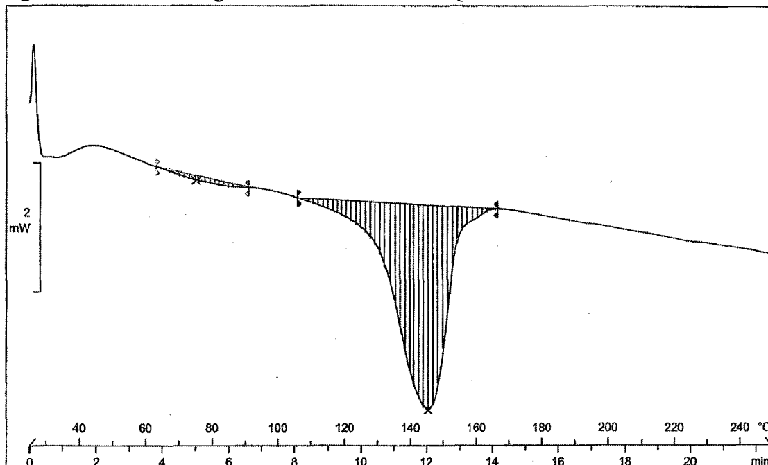
Figure 77: DSC thermogram of Dasatinib form AQ
