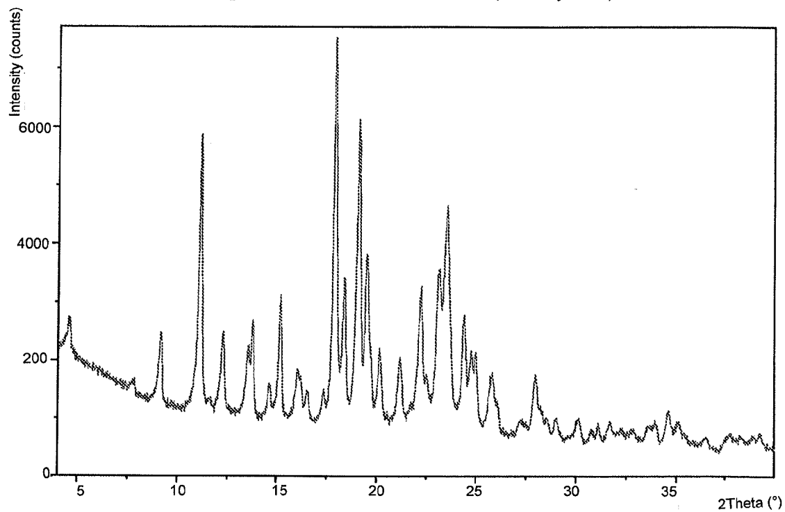
Figure 14: PXRD pattern of Dasatinib form H1-7 (monohydrate)
