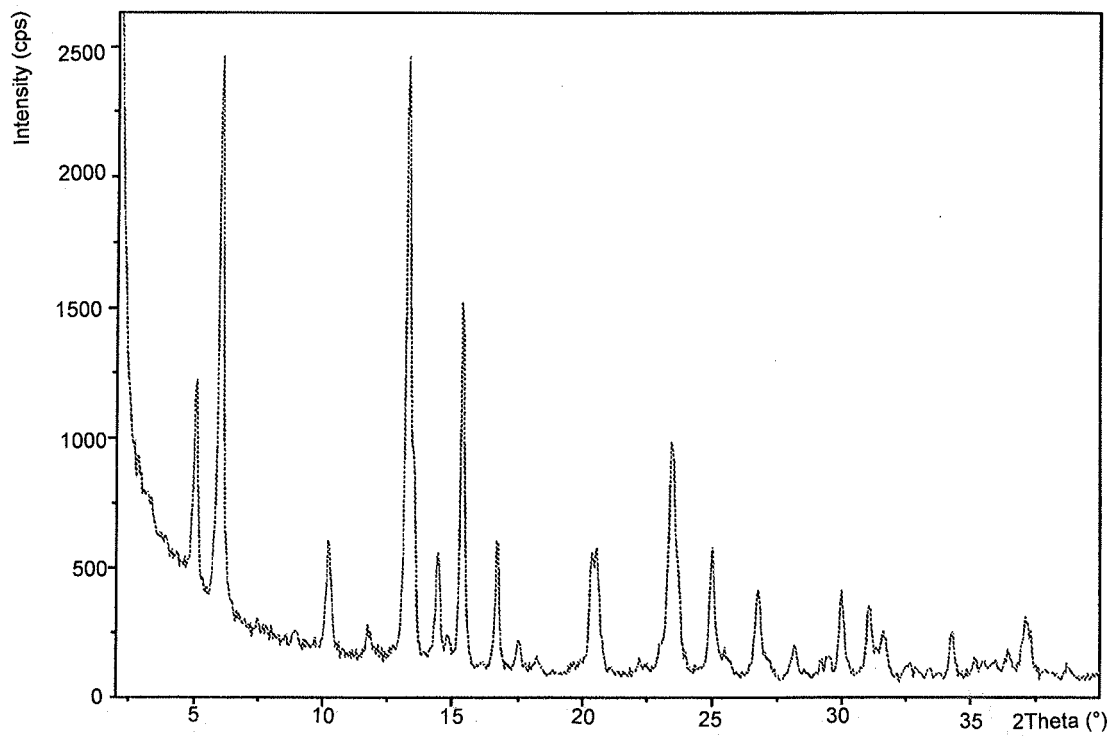
Figure 97: PXRD pattern of Dasatinib form BA
