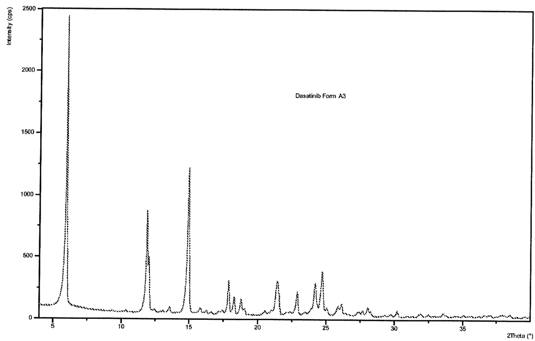
Figure 18: PXRD pattern of Dasatinib form A3
