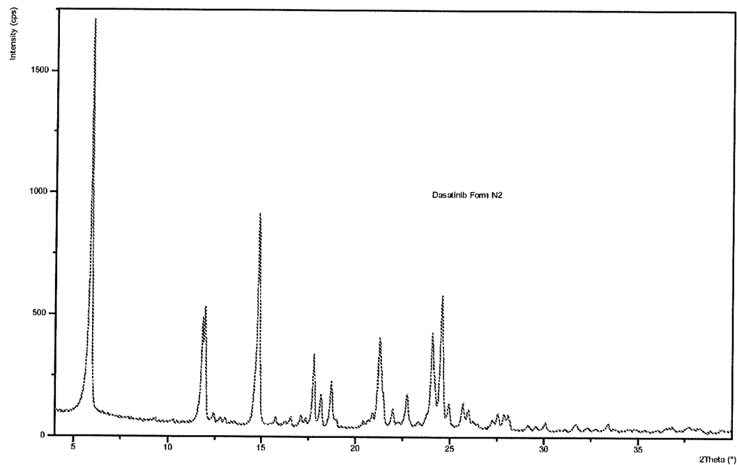
Figure 23: PXRD pattern of Dasatinib form N2
