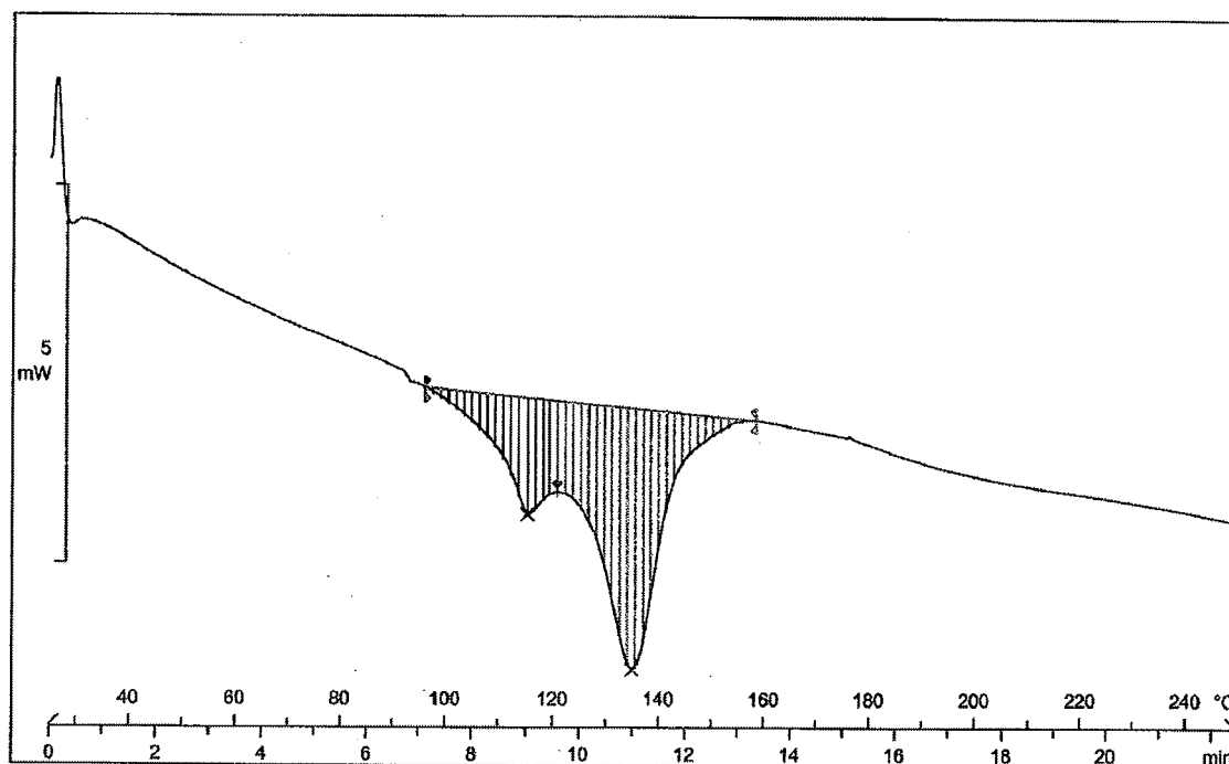
Figure 85: DSC thermogram of Dasatinib form AU
