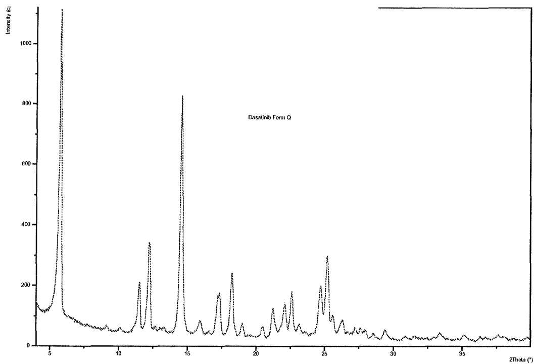
Figure 25: PXRD pattern of Dasatinib form Q
