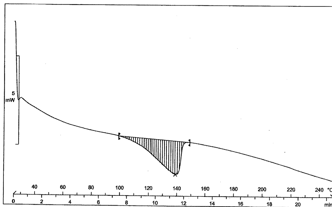
Figure 75: DSC thermogram of Dasatinib form AP
