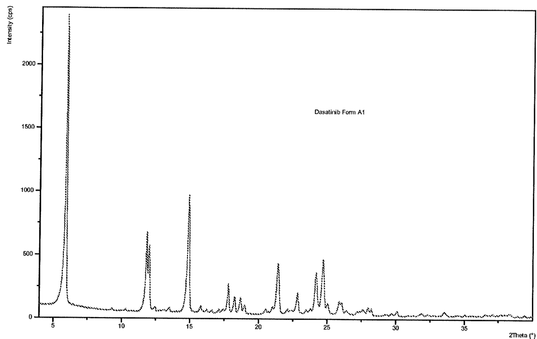
Figure 17: PXRD pattern of Dasatinib form A1
