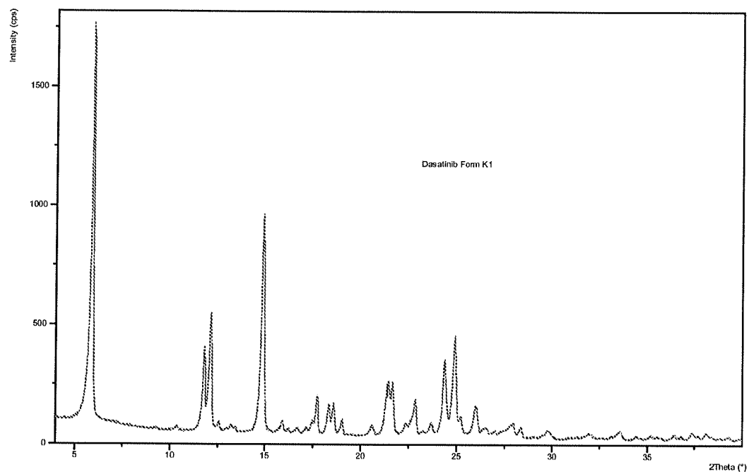
Figure 19: PXRD pattern of Dasatinib form K1
