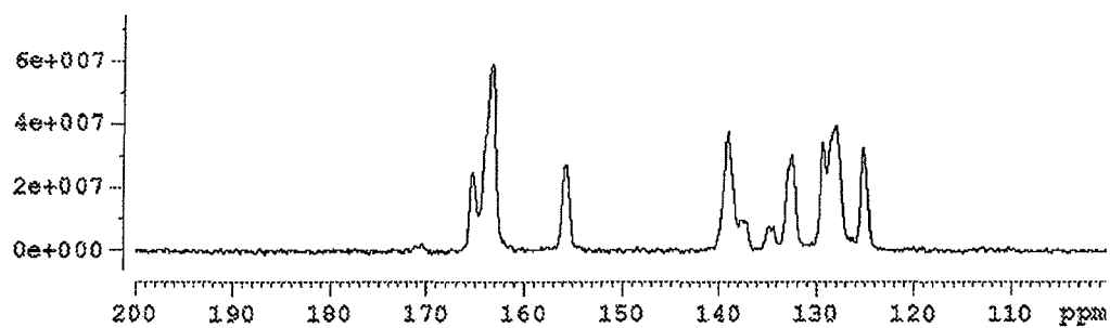
Figure 121: A full-width solid state ^{13}\text{C} NMR spectrum of dasatinib form A3.
