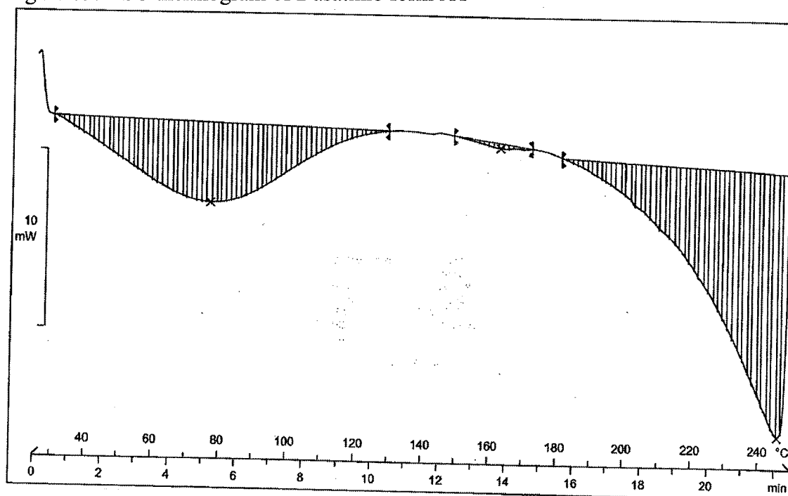
Figure 83: DSC thermogram of Dasatinib form AT
