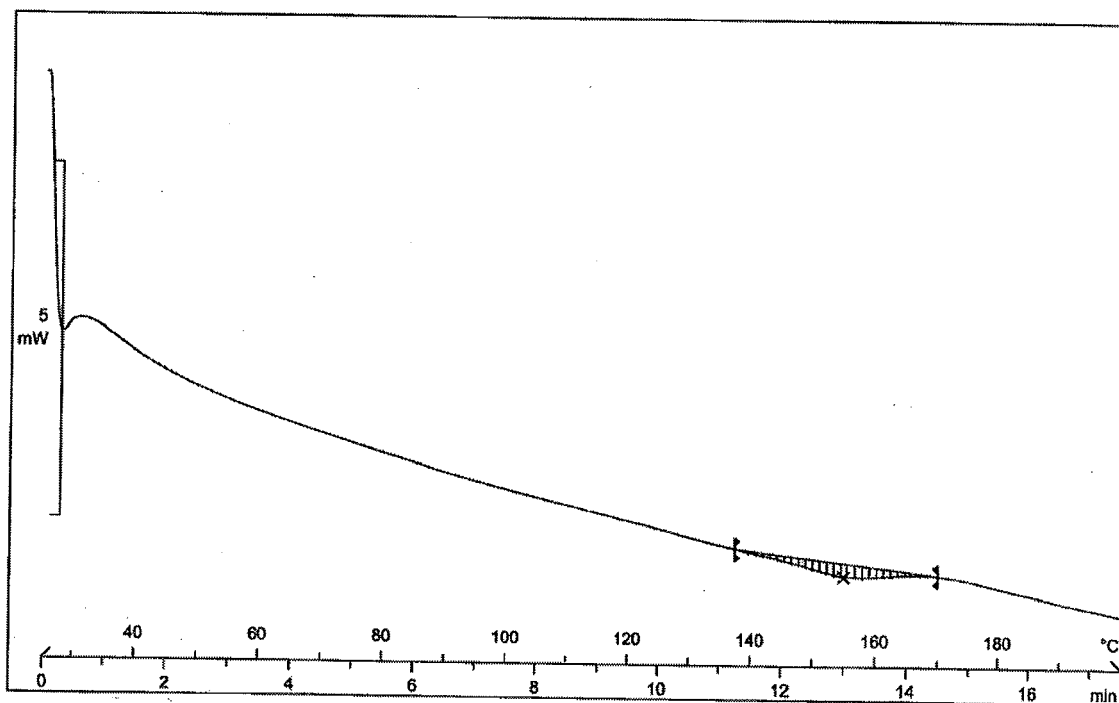
Figure 63: DSC thermogram of Dasatinib form AI
