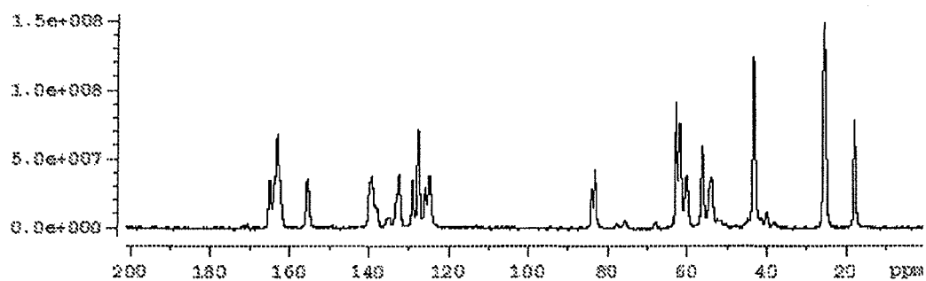
Figure 122: A detailed solid state ^{13}\text{C} NMR spectrum of dasatinib form A3.
