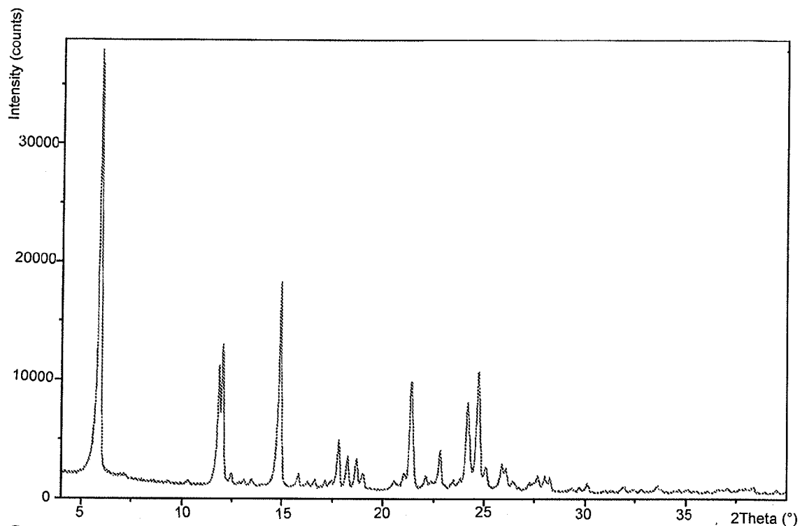
Figure 2: PXRD pattern of Dasatinib form B
