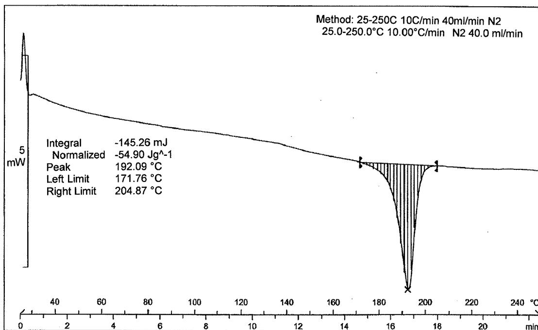
Figure 101: DSC thermogram of Dasatinib form BA
