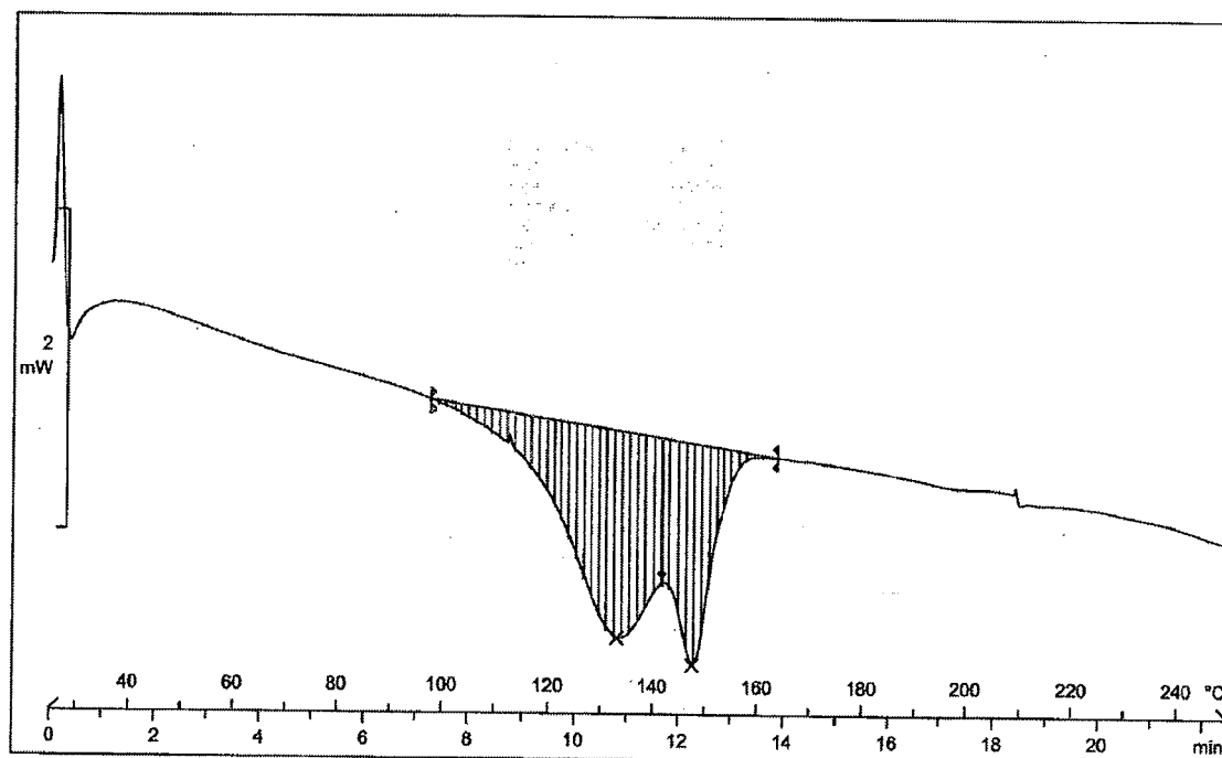
Figure 91: DSC thermogram of Dasatinib form AY
