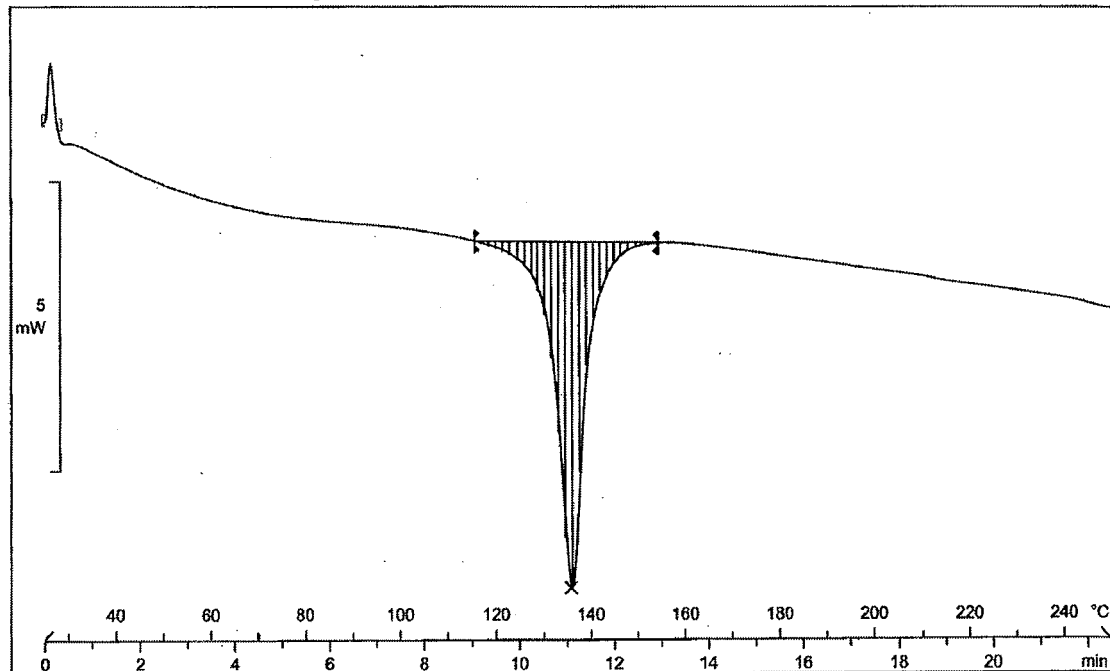
Figure 81: DSC thermogram of Dasatinib form AS
