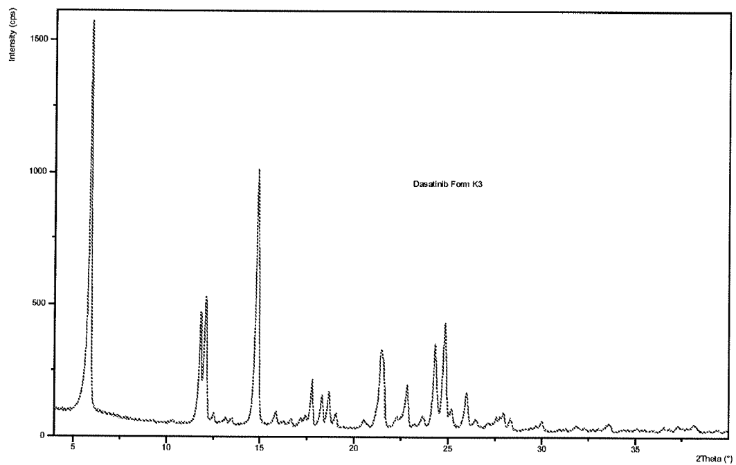
Figure 20: PXRD pattern of Dasatinib form K3
