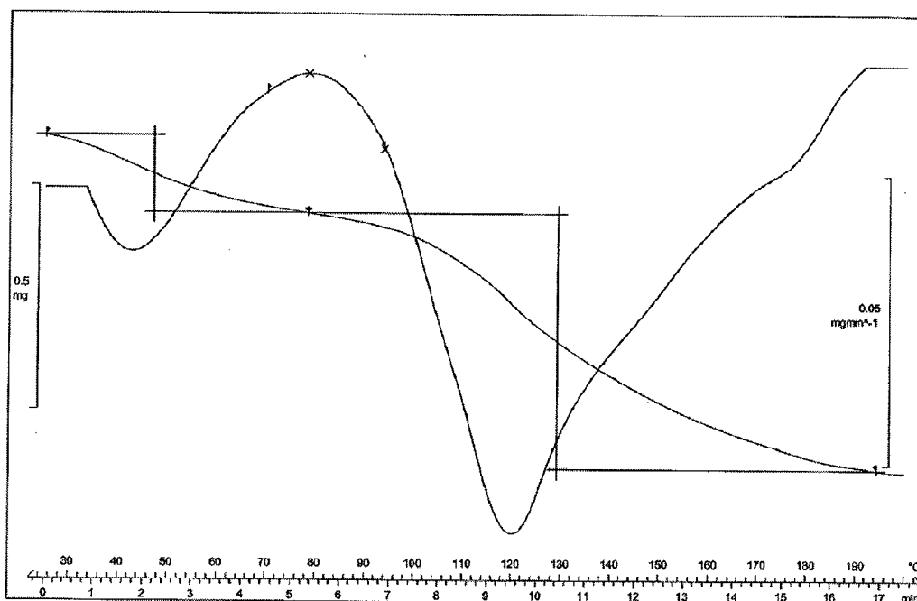
Figure 70: TGA thermogram of Dasatinib form AM
