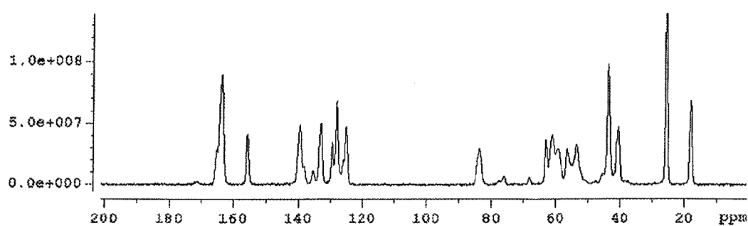
Figure 124: A detailed solid state ^{13}\text{C} NMR spectrum of dasatinib form A21.
