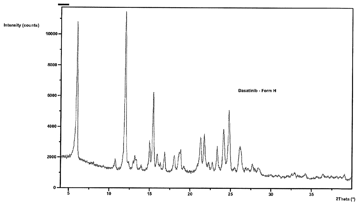
Figure 8: PXRD pattern of Dasatinib form H
