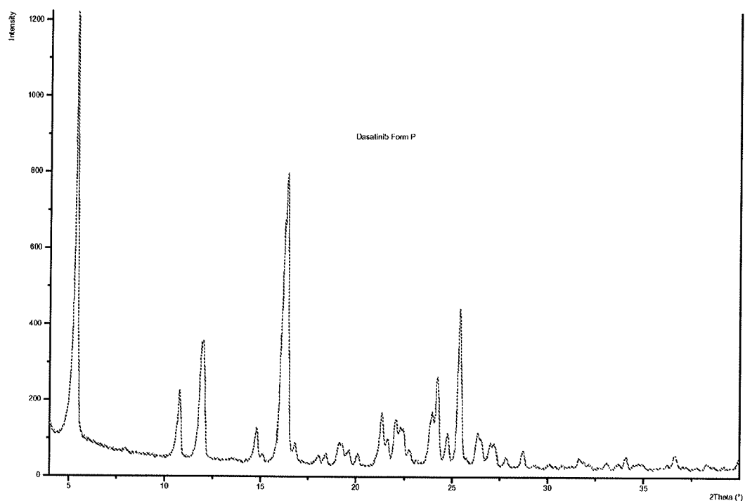
Figure 24: PXRD pattern of Dasatinib form P
