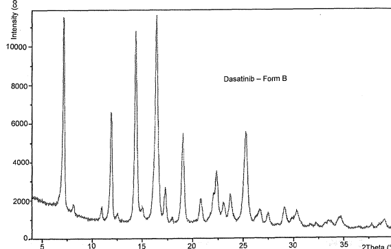
Figure 2: PXRD pattern of Dasatinib form B
