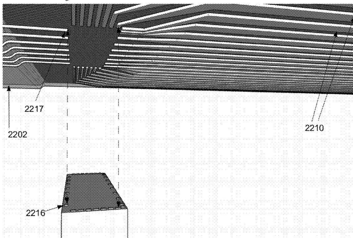
Fig 23e- IC COF attach
