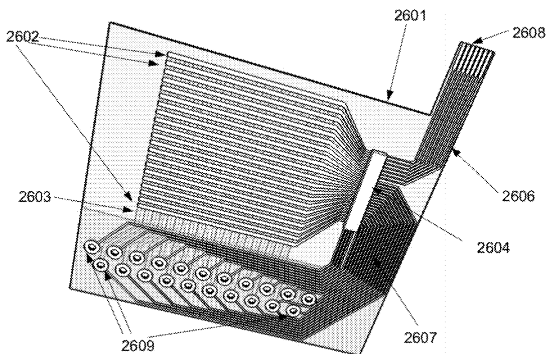
Figure 26b: Single Chip- Bottom View
