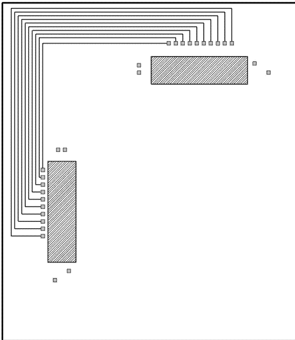
Fig 25C (Two Chip Sensor Substrate Top layer)
