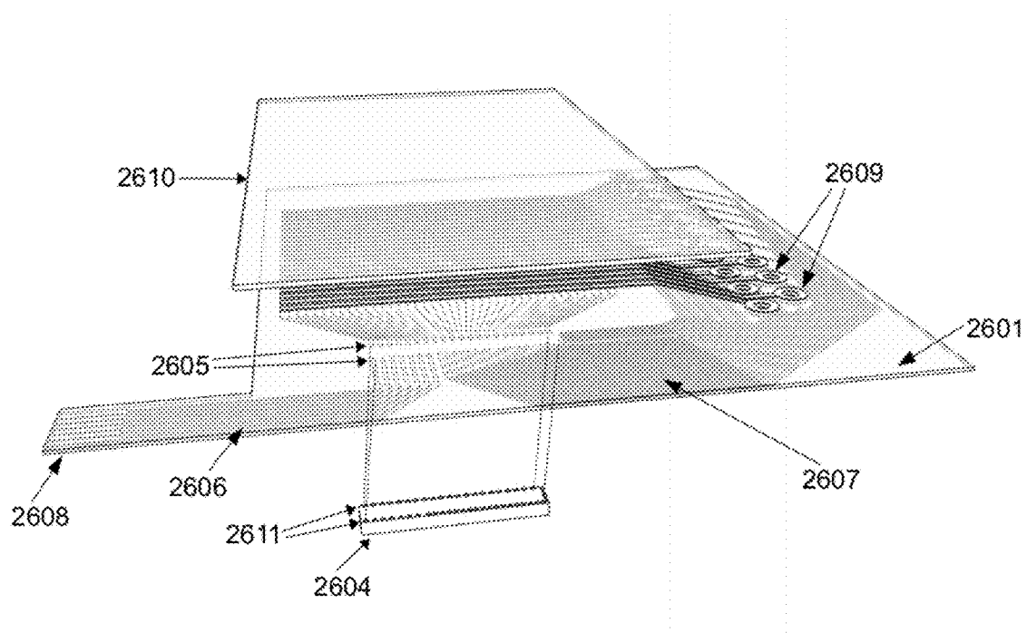
Fig 26c- Exploded View
