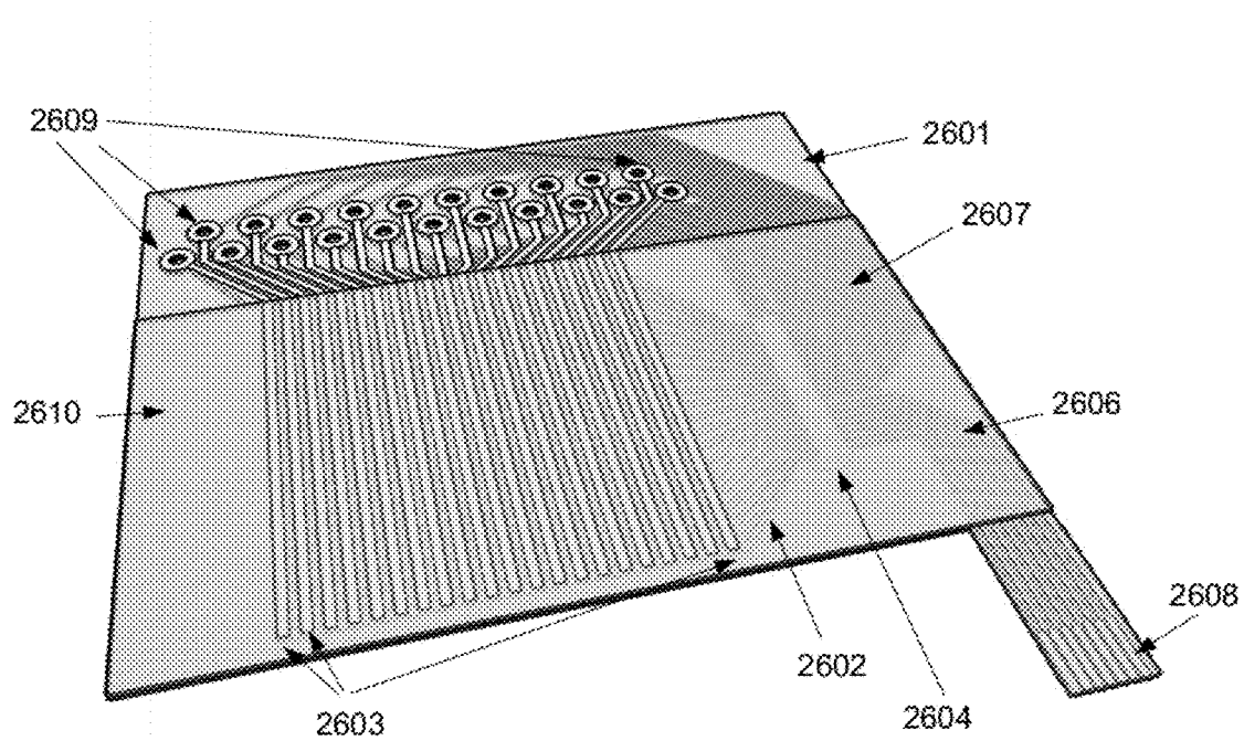
Figure 26a: Single Chip- Top View
