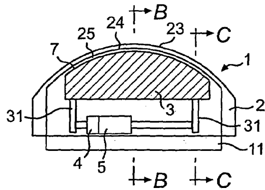
FIG. 5 PRIOR ART
