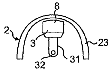
FIG. 7 PRIOR ART
