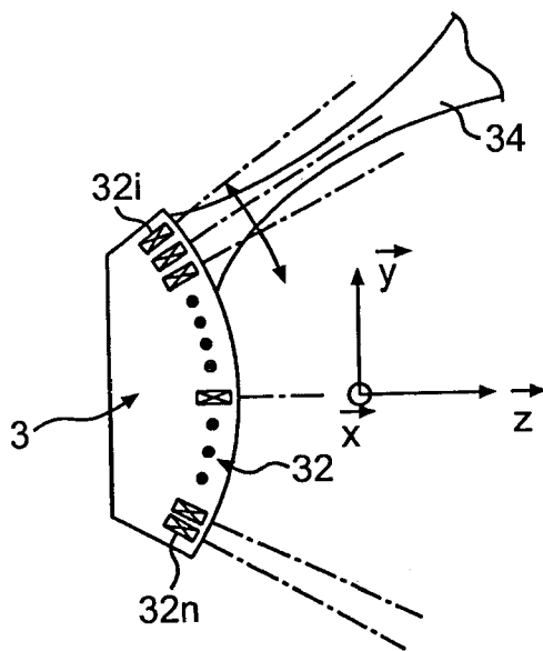
FIG. 3 PRIOR ART
