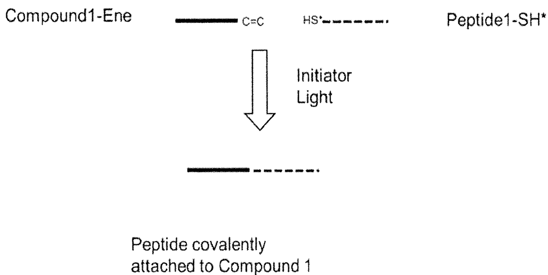
D – Derivatized polypeptide
