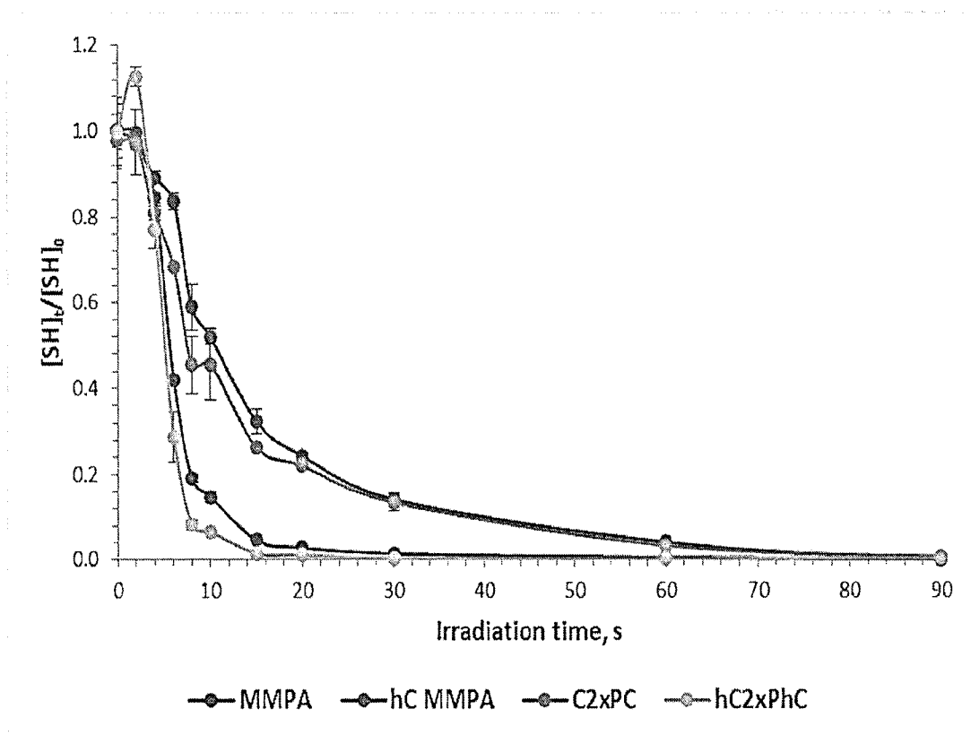
B – Consumption of thiol groups for peptide amino acids
