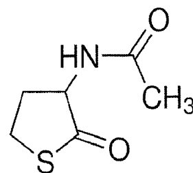
F - N-acetyl homocysteine thiolactone
