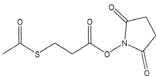
E - N-succinimidyl-S-acetylthiopropionate (SATP)
