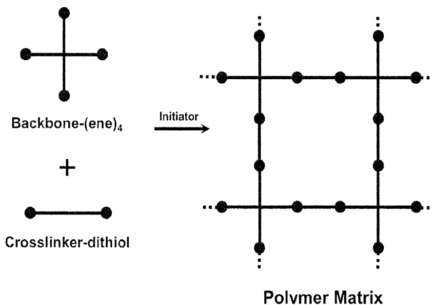
A – Sample Thiol-ene polymer matrix
