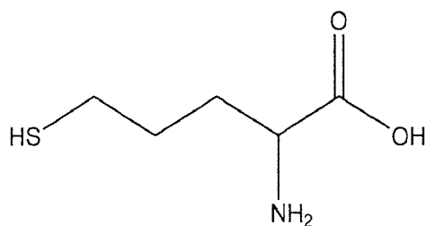
C - 2-amino-5-mercaptopentanoic acid
