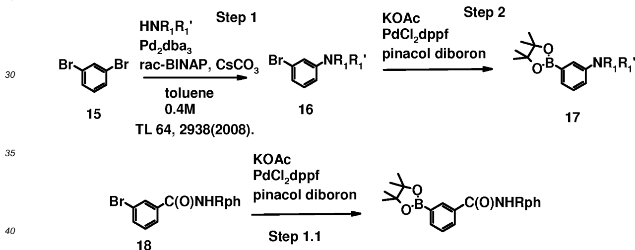
Scheme 8: boronic acid pinacol ester formation.
