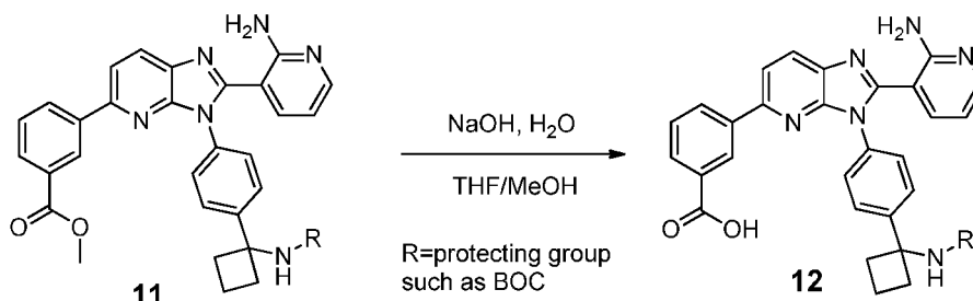
Scheme 5: Saponification
