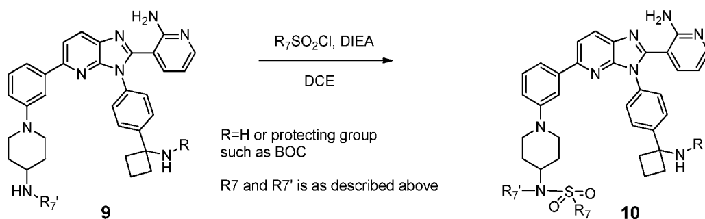
Scheme 4: Sulfonamide formation
