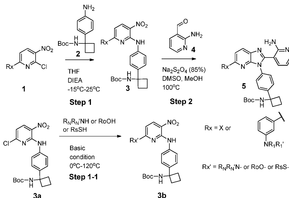
Scheme 1: Imidazopyridine formation and N,S,O substitution on pyridine
