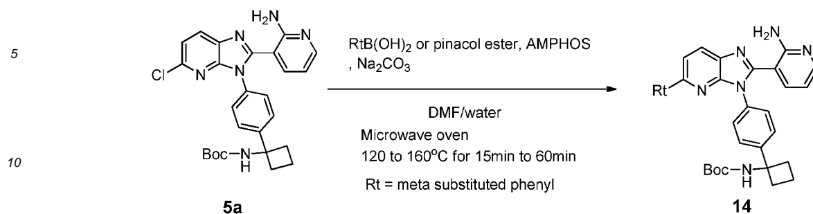
Scheme 7: Suzuki coupling 2
