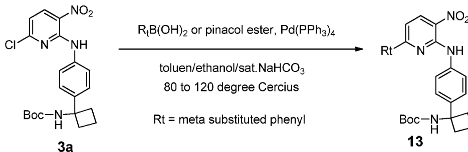
Scheme 6: Suzuki coupling 1
