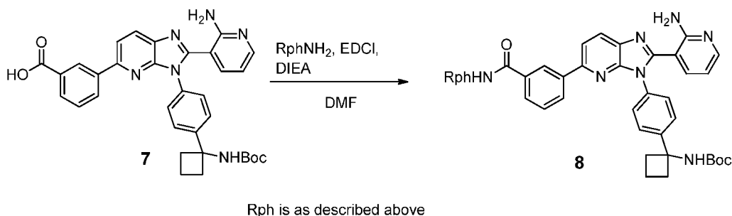
Scheme 3: Amido formation
