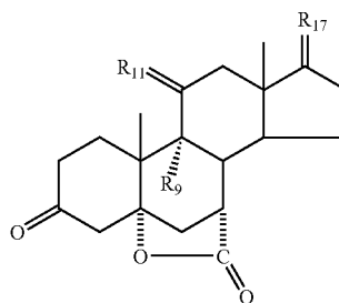
(VII-unprotected A-ring)
