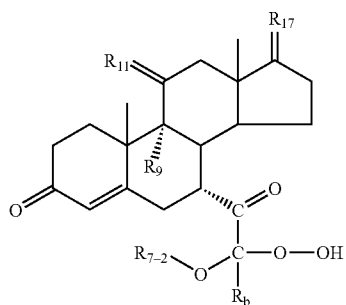
(IV-OOH-unprotected A-ring)
