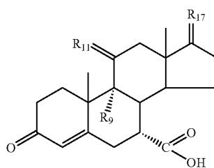
(V-unprotected A-ring)
