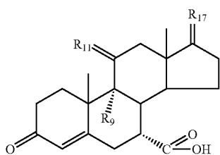
(VI-unprotected A-ring)
