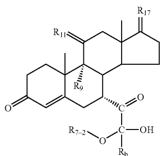
(IV-OH-unprotected A-ring)
