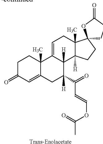
Trans-Enolacetate
