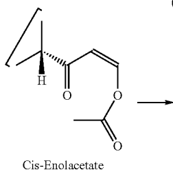
Cis-Enolacetate
