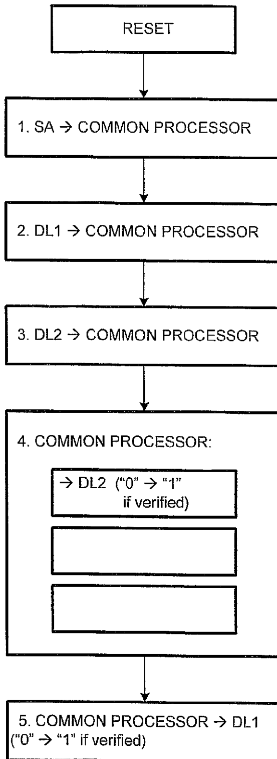
PROGRAM VERIFY OPERATION (2-bit program)
