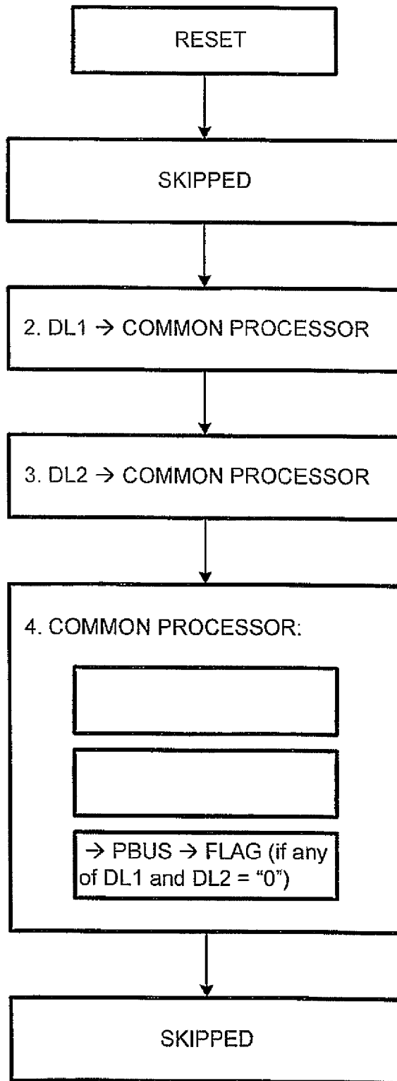
ERROR DETECTION (2-bit program)
