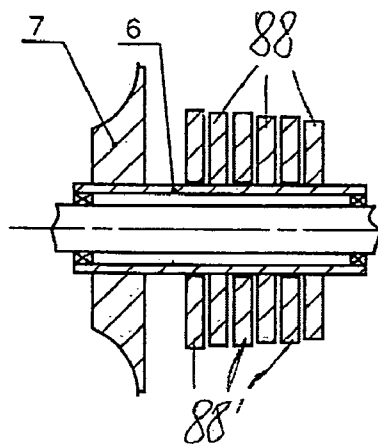
Figure 4 – Axial construction (variant)
