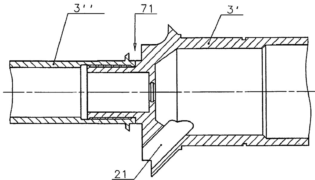
Figure 7 – Supporting hollow shafts
