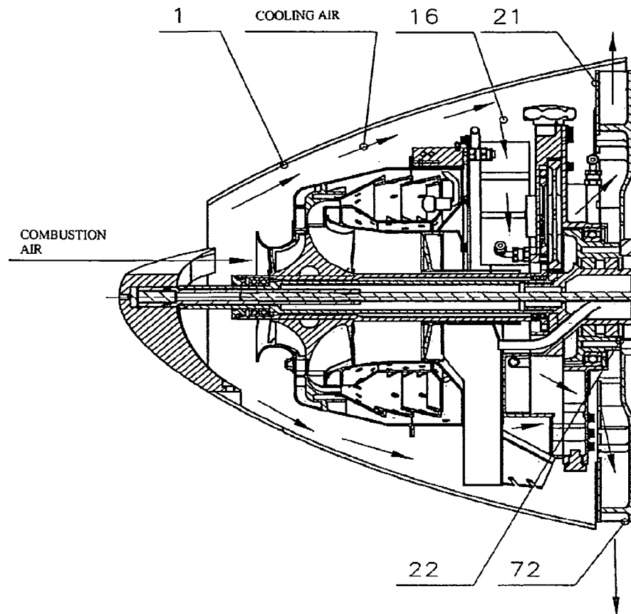
Figure 10 – Cooling-air flow
