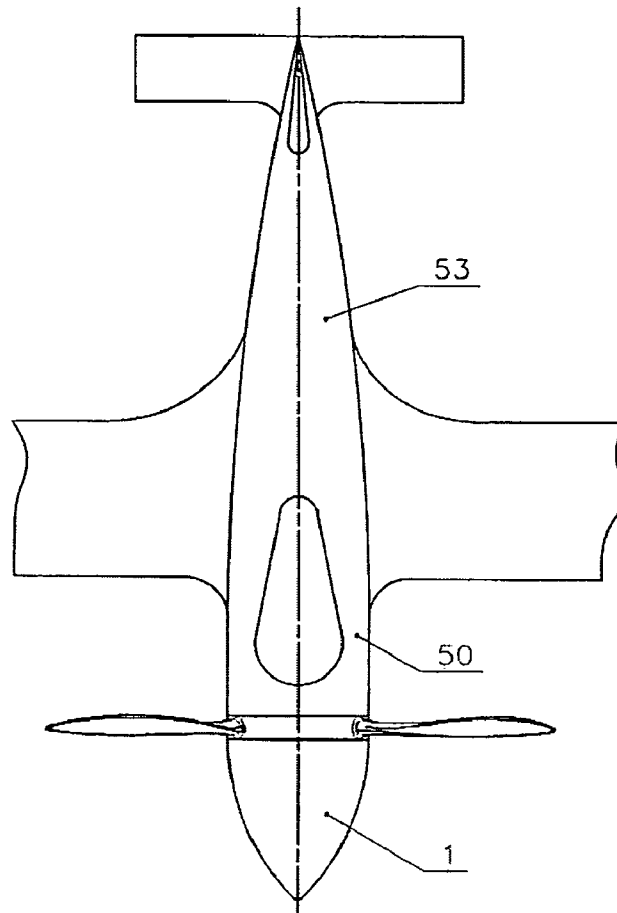
Figure 1 – Drive unit for propeller-driven aeroplanes
