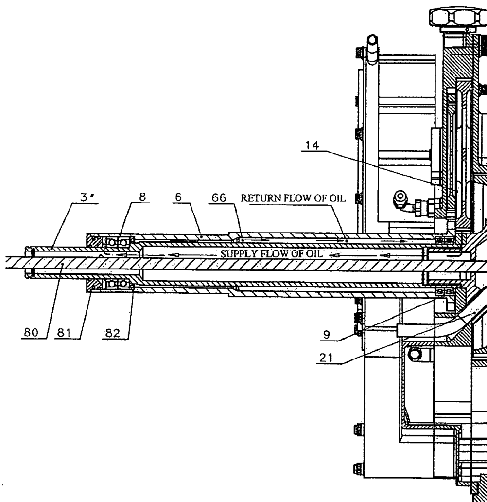
Figure 5 – Mounting and oil circuit
