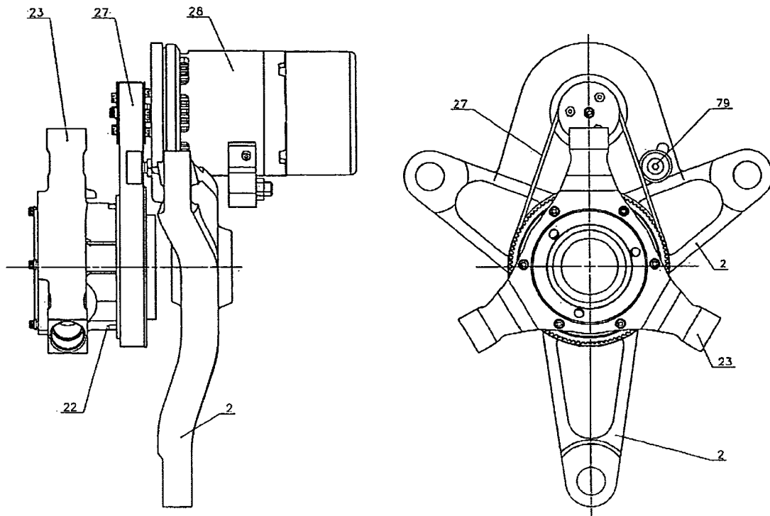
Figure 12 – Starter / generator unit
