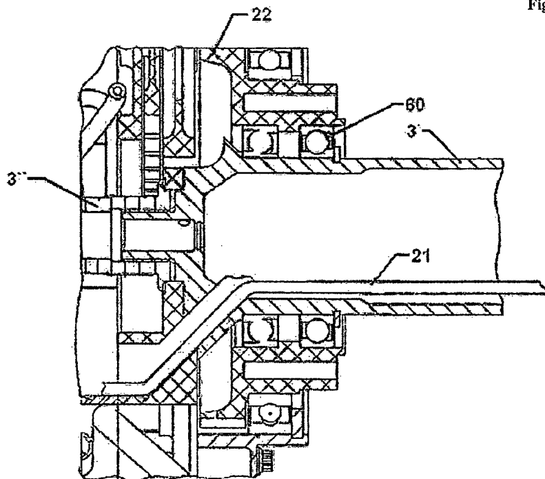
Figure 9 – Leading-through of the supply lines
