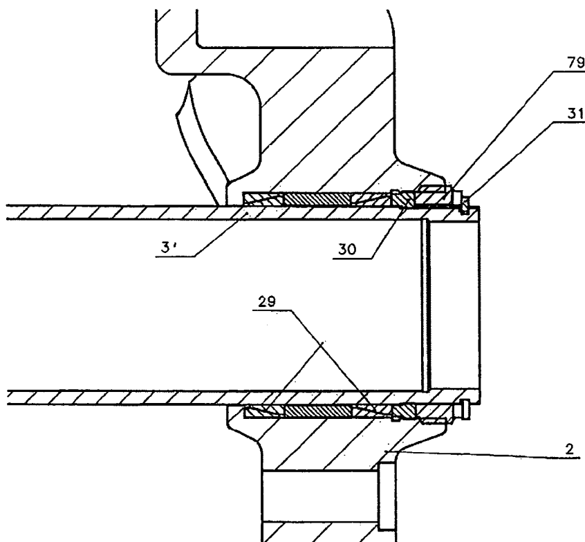
Figure 13 – Fixing system
