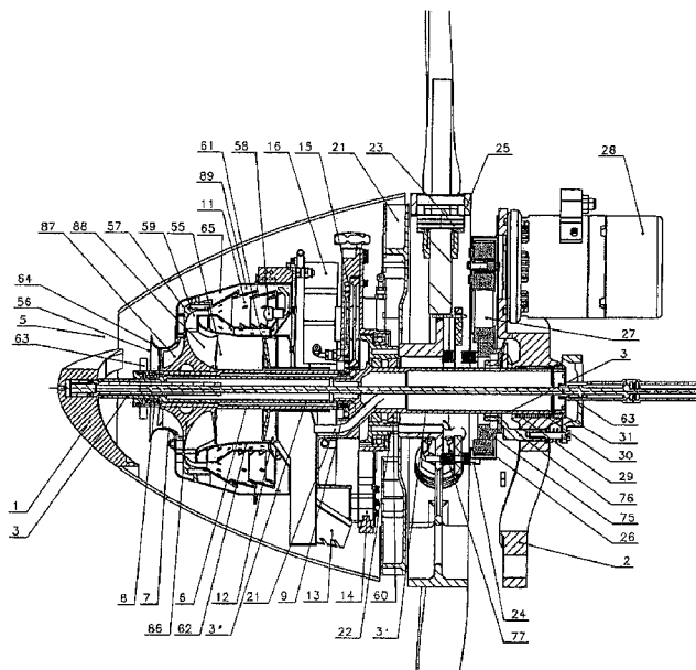
Overall illustration of drive unit
