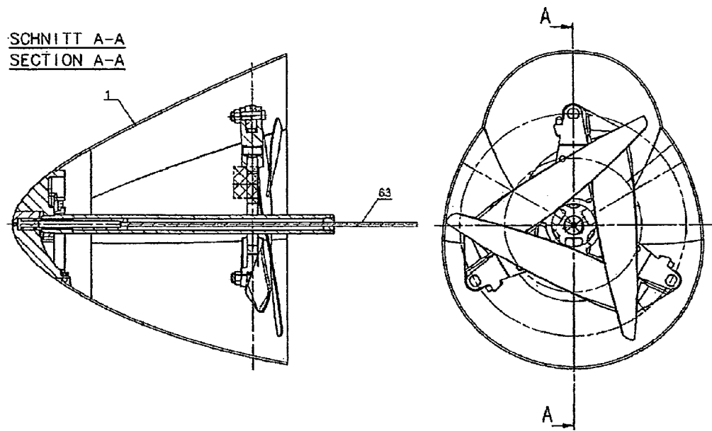
Figure 15a – Folding propeller closed
