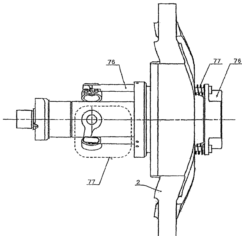
Figure 11 – Propeller-adjustment device
