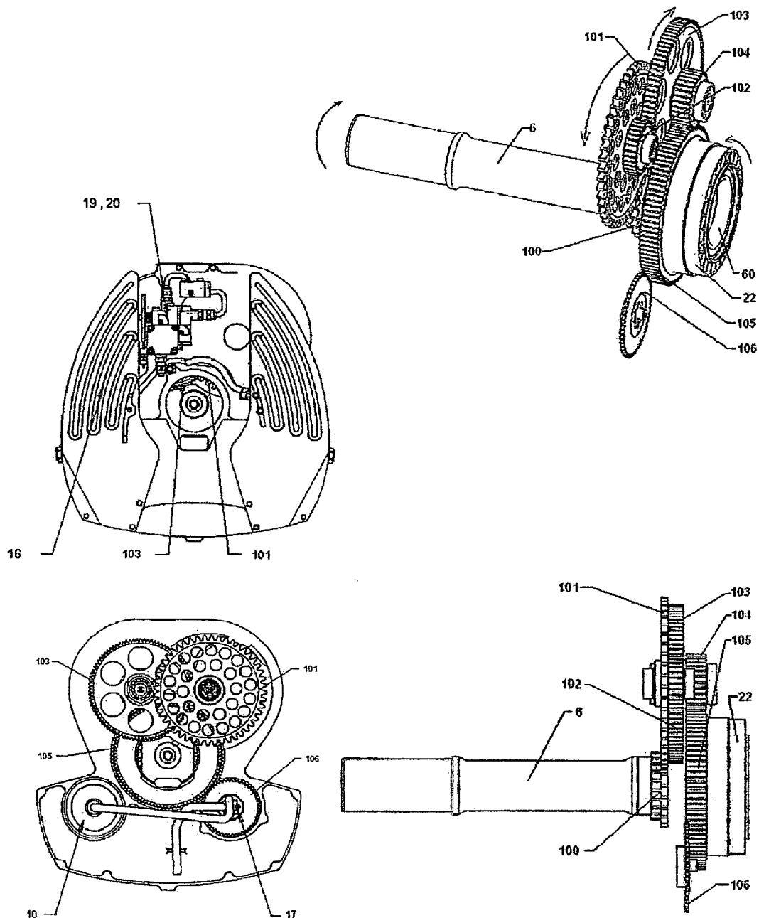
Figure 8b – Gear stages and oil pump
