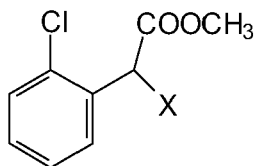
X = Cl or Br Formula III
