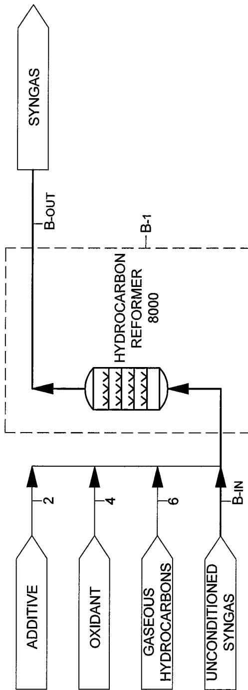
FIGURE 2 STEP B, HYDROCARBON REFORMING
