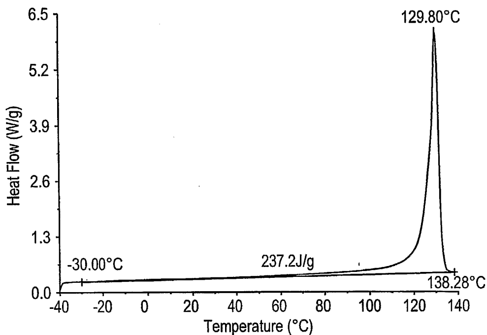
FIG. 23 DSC Comparative B*
