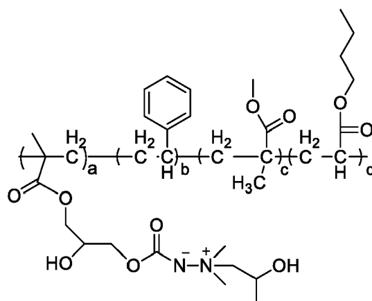
(formula XI).
