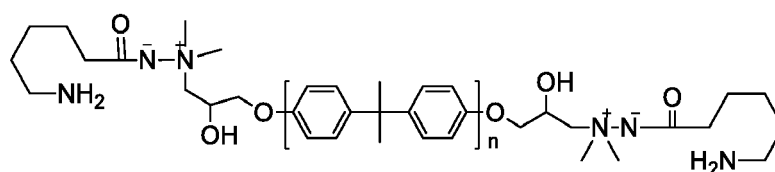
25 (formula IX);
