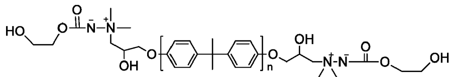
15 (formula VIII);
