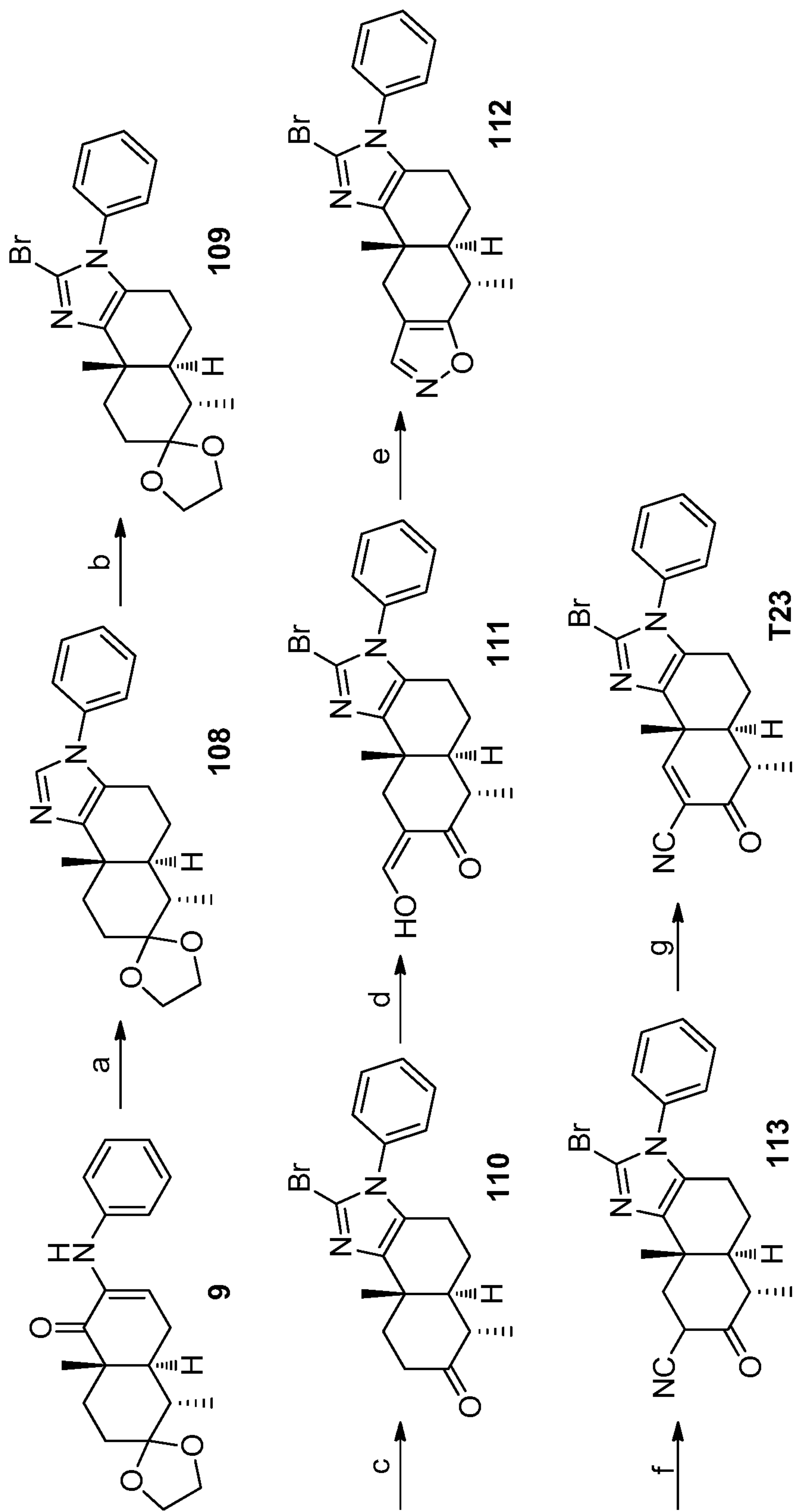
Scheme 20
