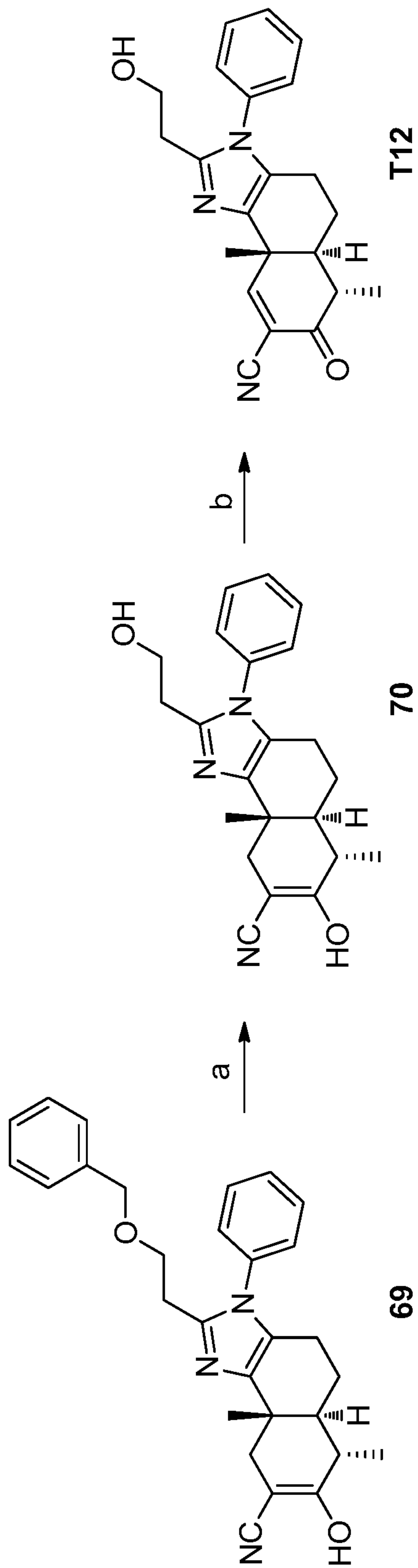
Scheme 12
