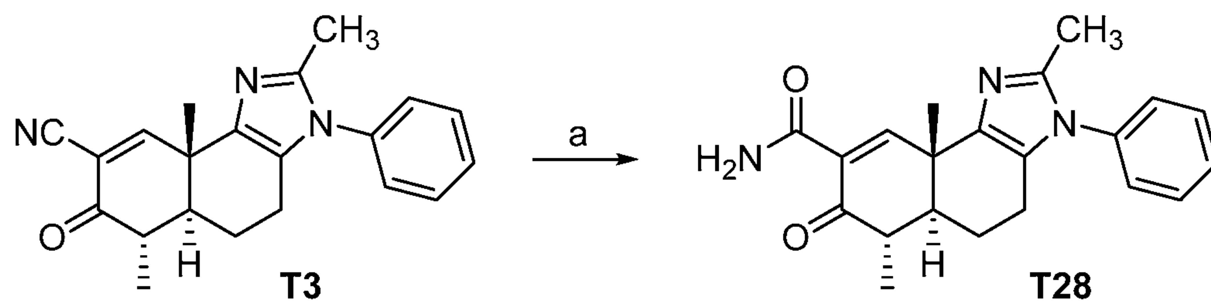
Scheme 24
