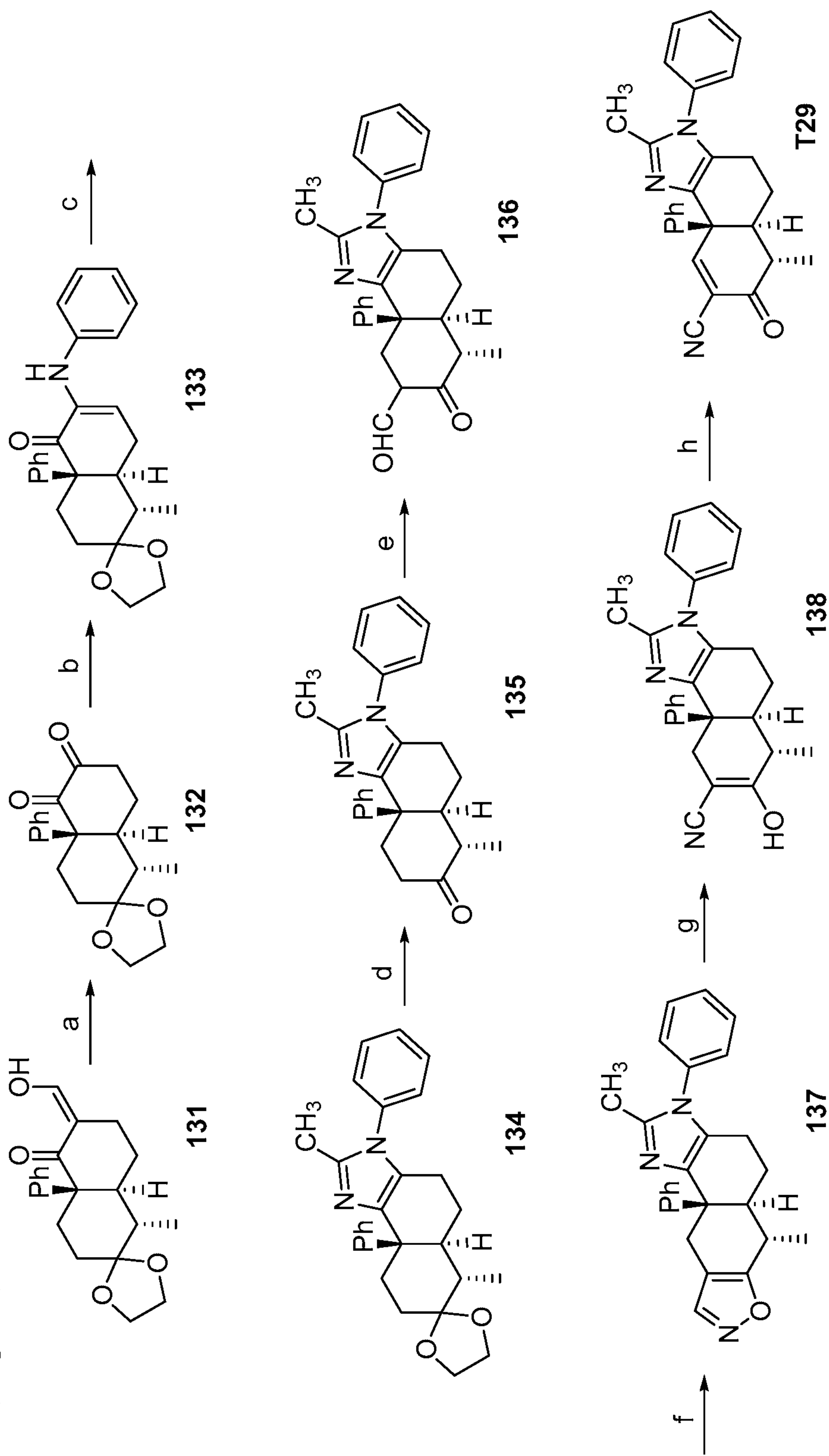
Scheme 25 (Proposed)
