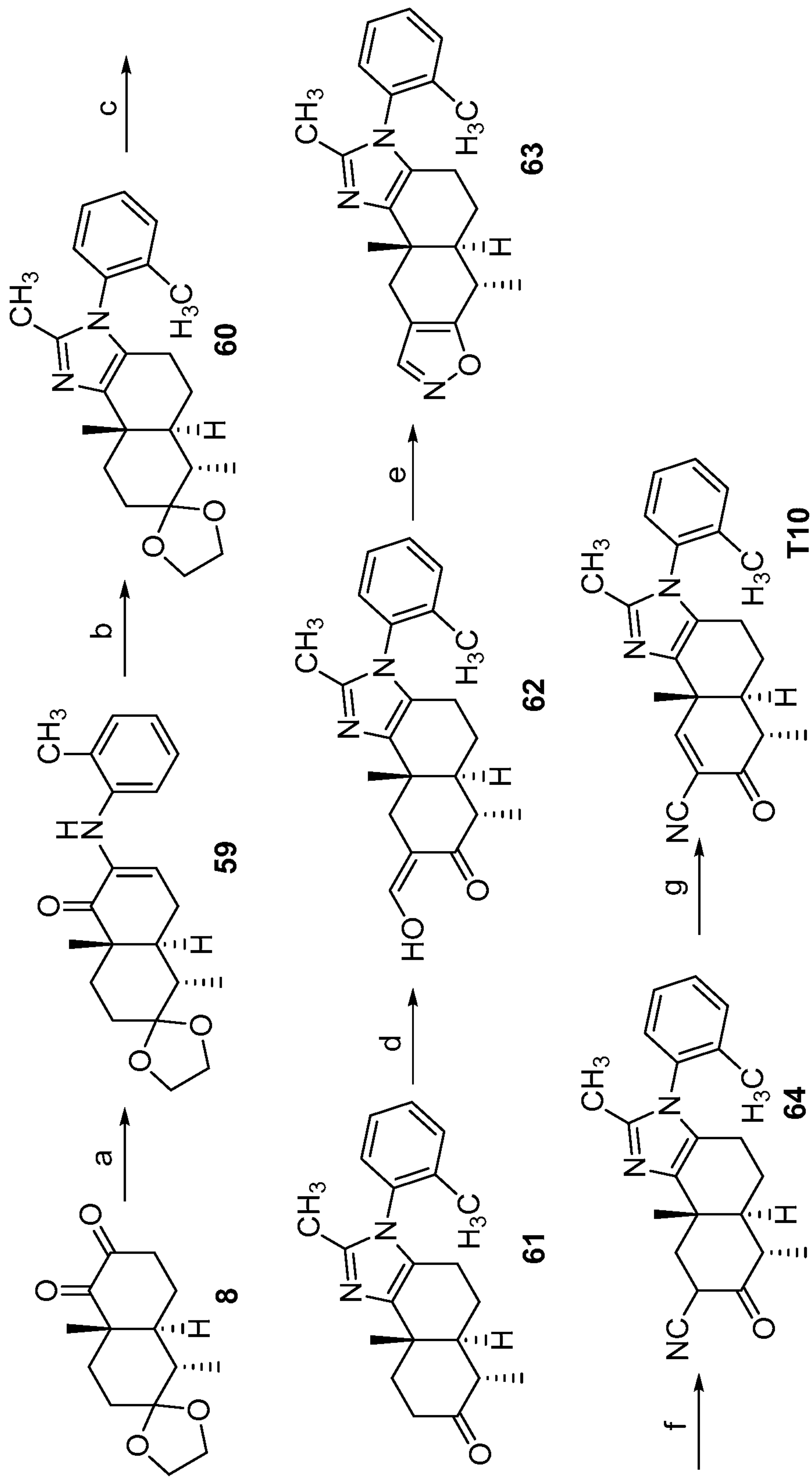
Scheme 10
