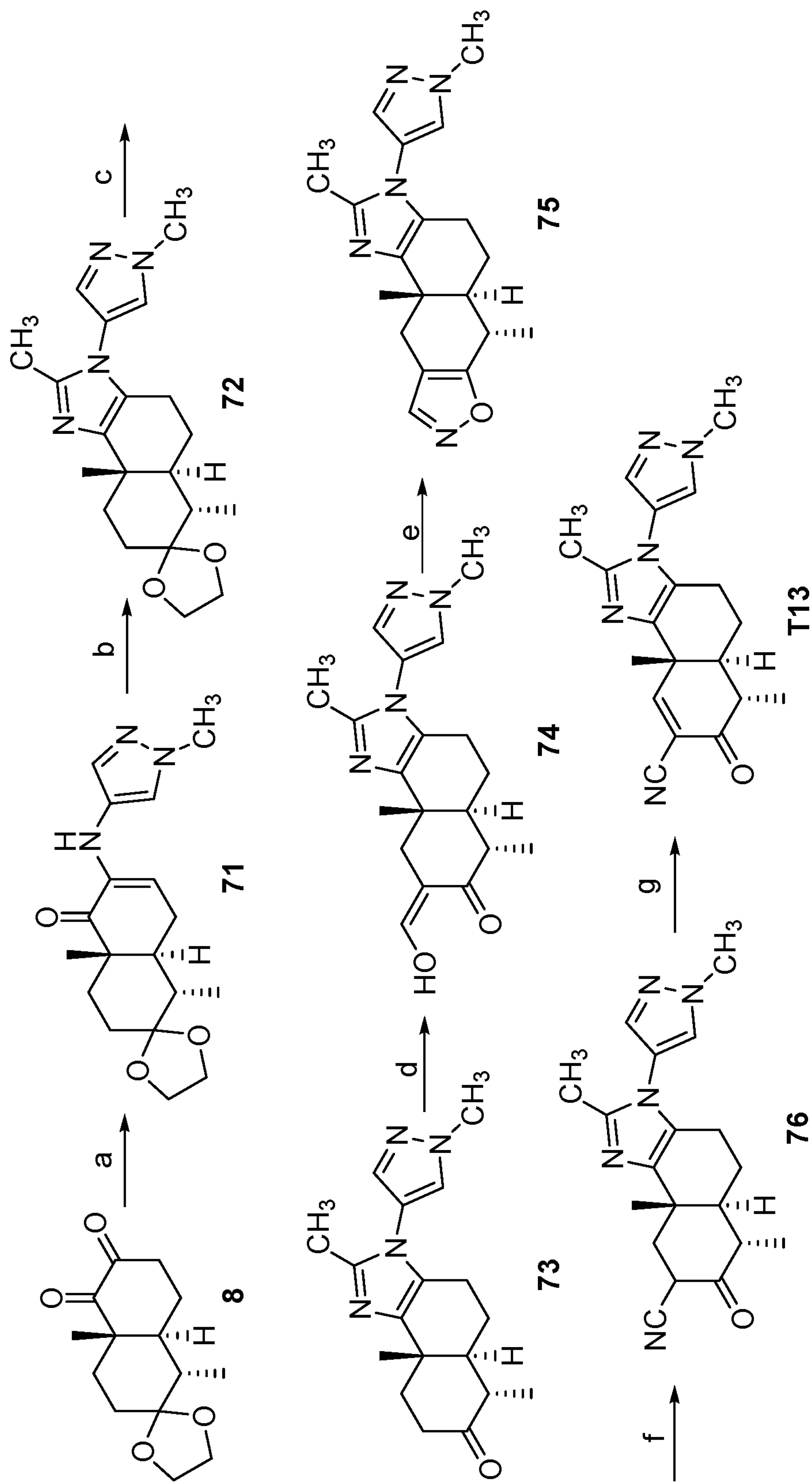
Scheme 13
