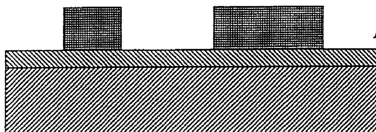
Removal of mask after evaporation of aluminum
