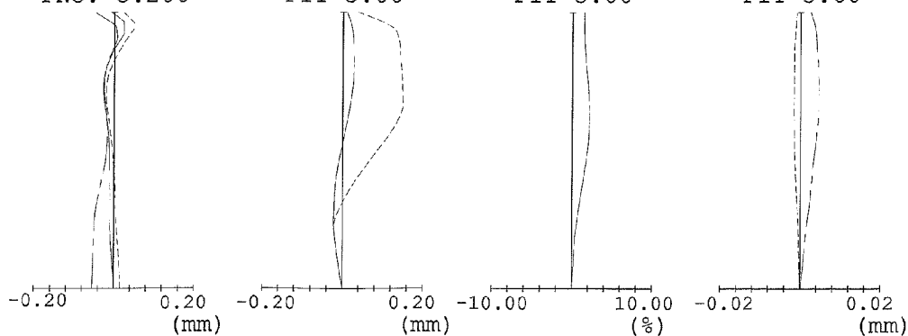
FIG. 18I FIG. 18J FIG. 18K FIG. 18L SPHERICAL ABERRATION ASTIGMATISM DISTORTION CHROMATIC ABERRATION OF FNO. 5.200 FIY 3.00 FIY 3.00 FIY 3.00 MAGNIFICATION
