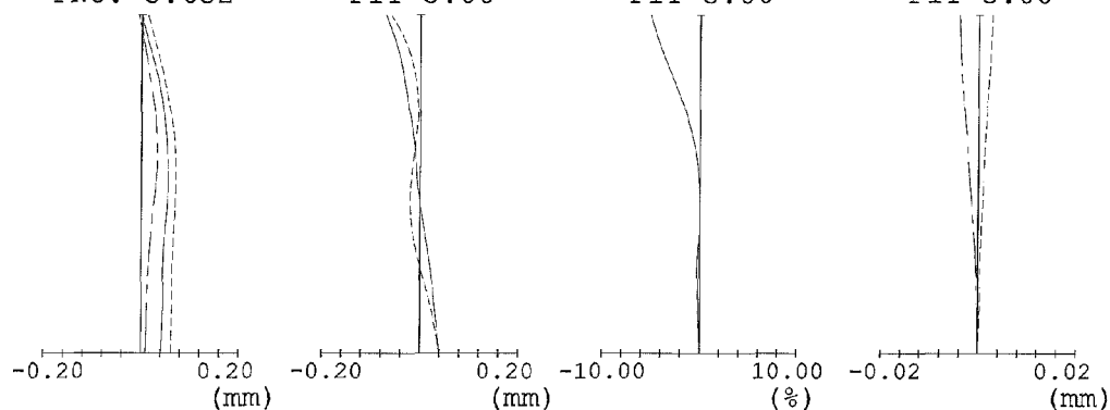
FIG.19E FIG.19F FIG.19G FIG.19H SPHERICAL ABERRATION FNO. 4.276 ASTIGMATISM FIY 3.00 DISTORTION FIY 3.00 CHROMATIC ABERRATION OF MAGNIFICATION FIY 3.00
