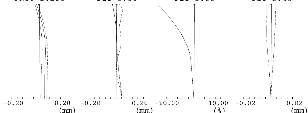
FIG. 18E FIG. 18F FIG. 18G FIG. 18H SPHERICAL ABERRATION ASTIGMATISM DISTORTION CHROMATIC ABERRATION OF FNO. 4.349 FIY 3.00 FIY 3.00 FIY 3.00 MAGNIFICATION
