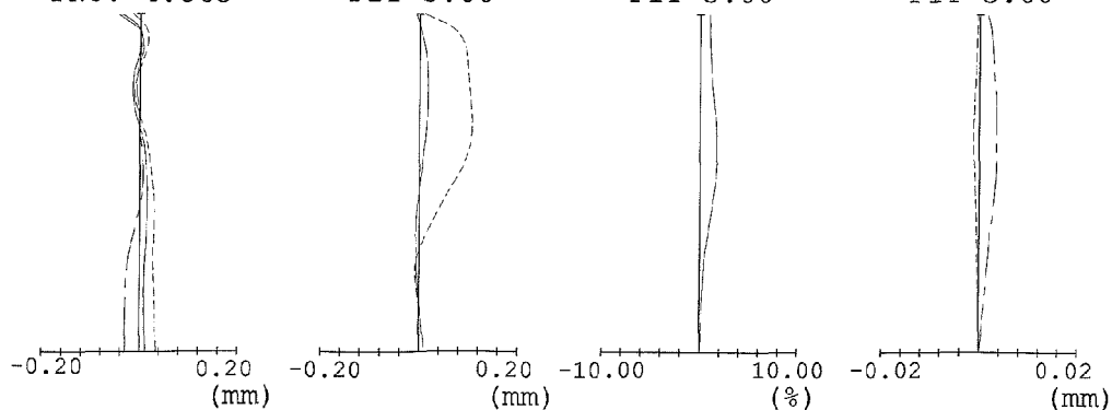
FIG.19I FIG.19J FIG.19K FIG.19L SPHERICAL ABERRATION FNO. 4.863 ASTIGMATISM FIY 3.00 DISTORTION FIY 3.00 CHROMATIC ABERRATION OF MAGNIFICATION FIY 3.00
