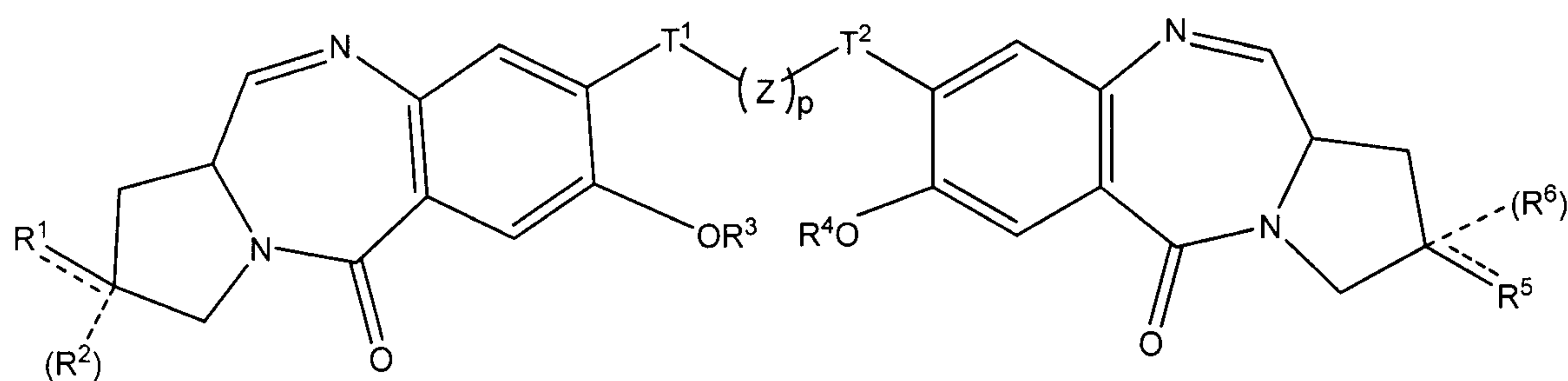
(Formula II)
