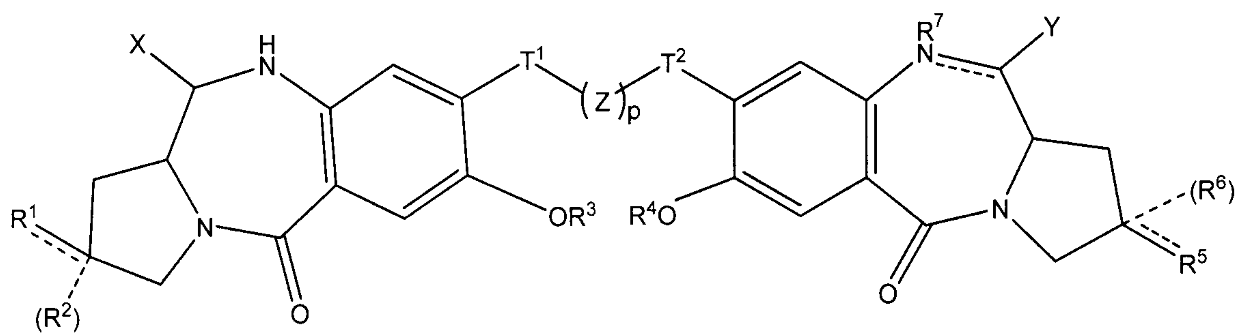
(Formula I)
