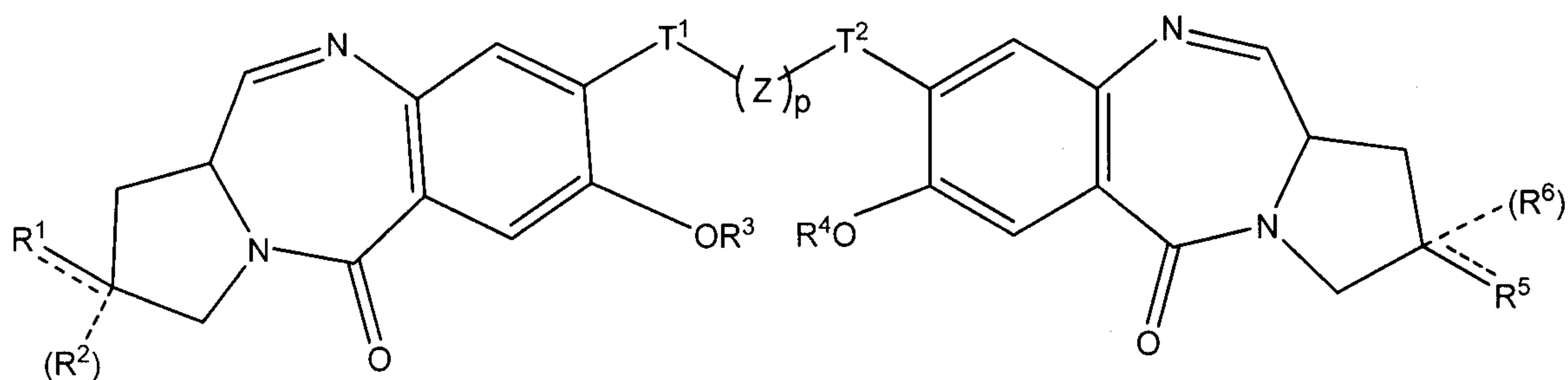
(Formula II)
