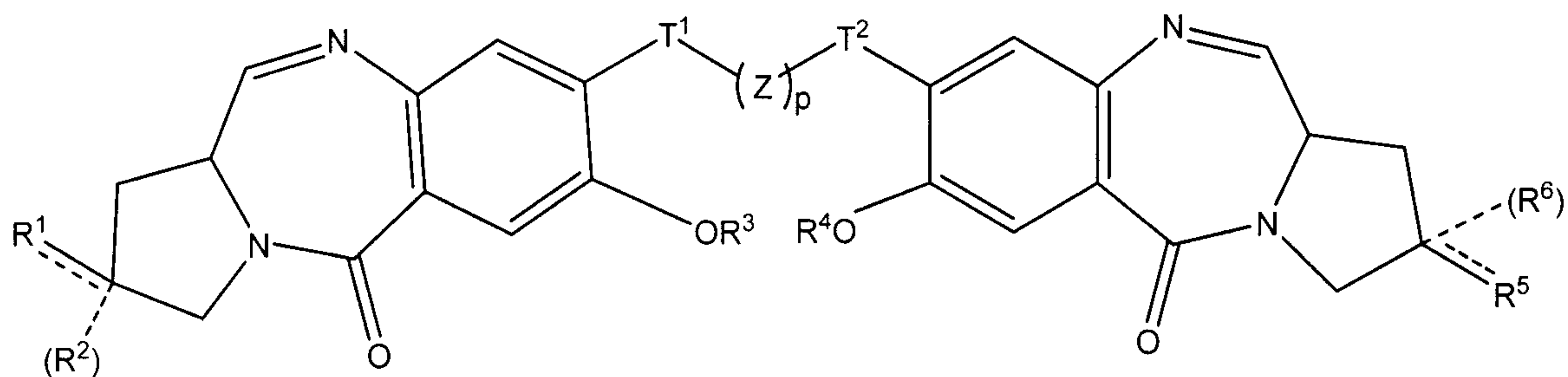
(Formula II)
