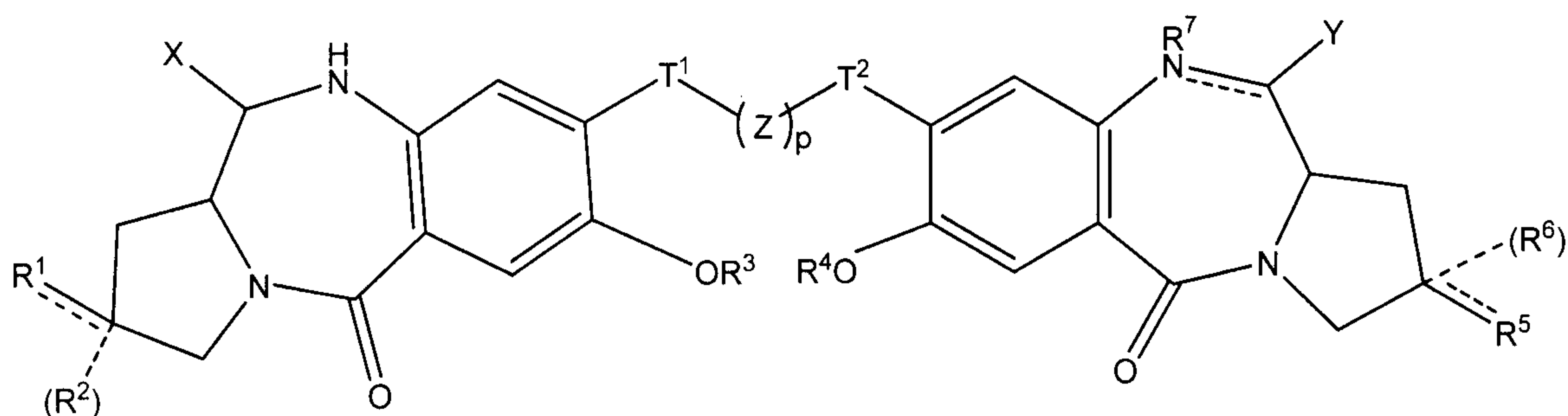
(Formula I)
