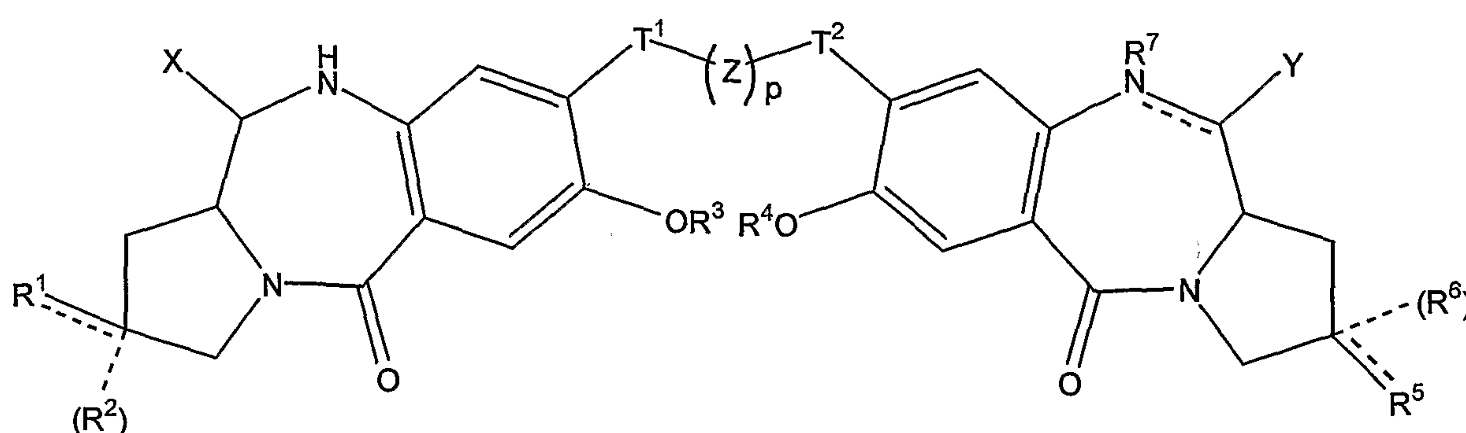
(Formula I)
