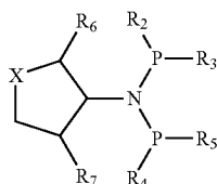
[Chemical Formula 1]
