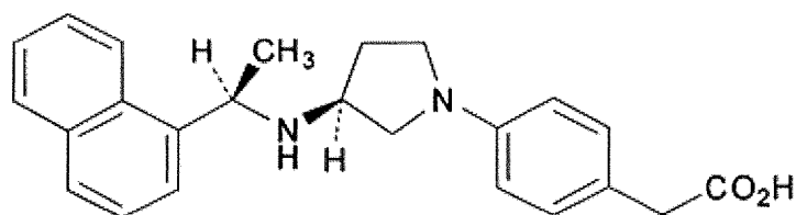
35 40 Compound A
