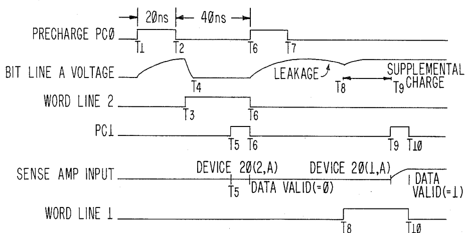
FIG. 3 TIMING DIAGRAM
