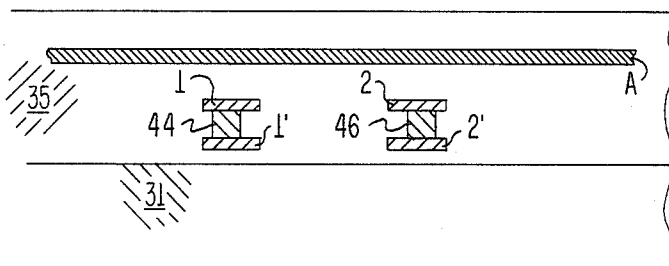
FIG. 5 SEC 5-5' (OF FIG. 2)
