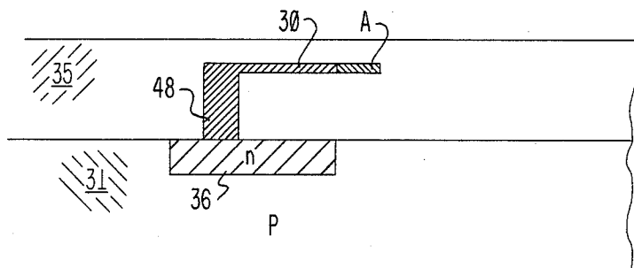
FIG. 6 SEC 6-6' (OF FIG. 2)
