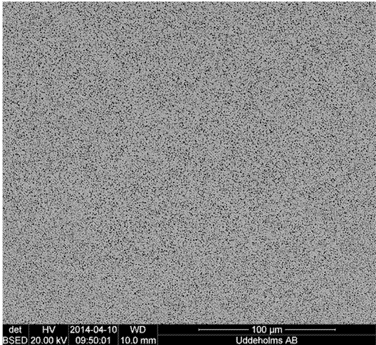
Figure 1. Microstructure of the inventive steel. Small and uniformly distributed MX-particles (black phase) in the steel matrix.
