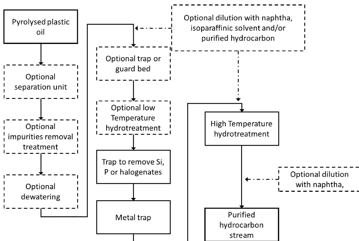
Figure 1. Overview of the possible process stream
