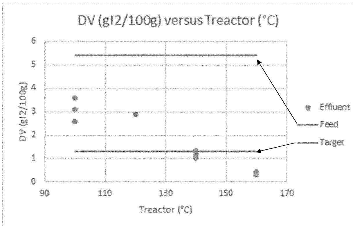
Figure 3: diene value as function of the temperature of the test in the case of example 3.
