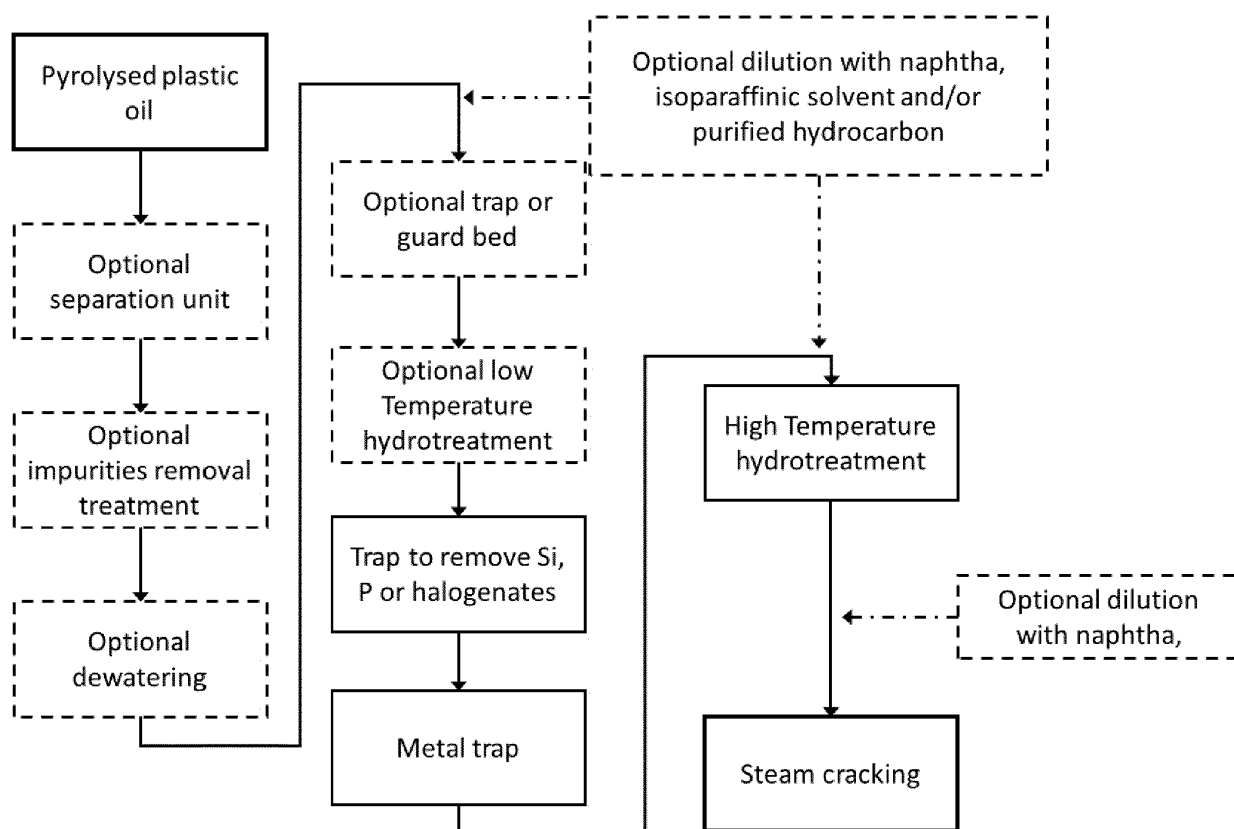
Figure 2. Overview of the possible process stream and application
