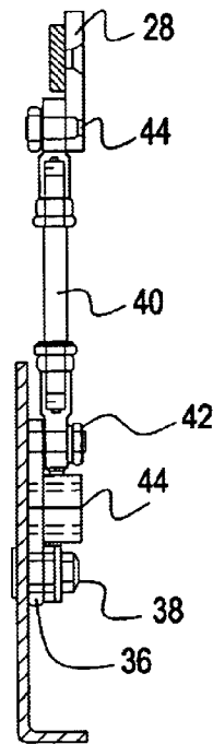
SECTION B-B
