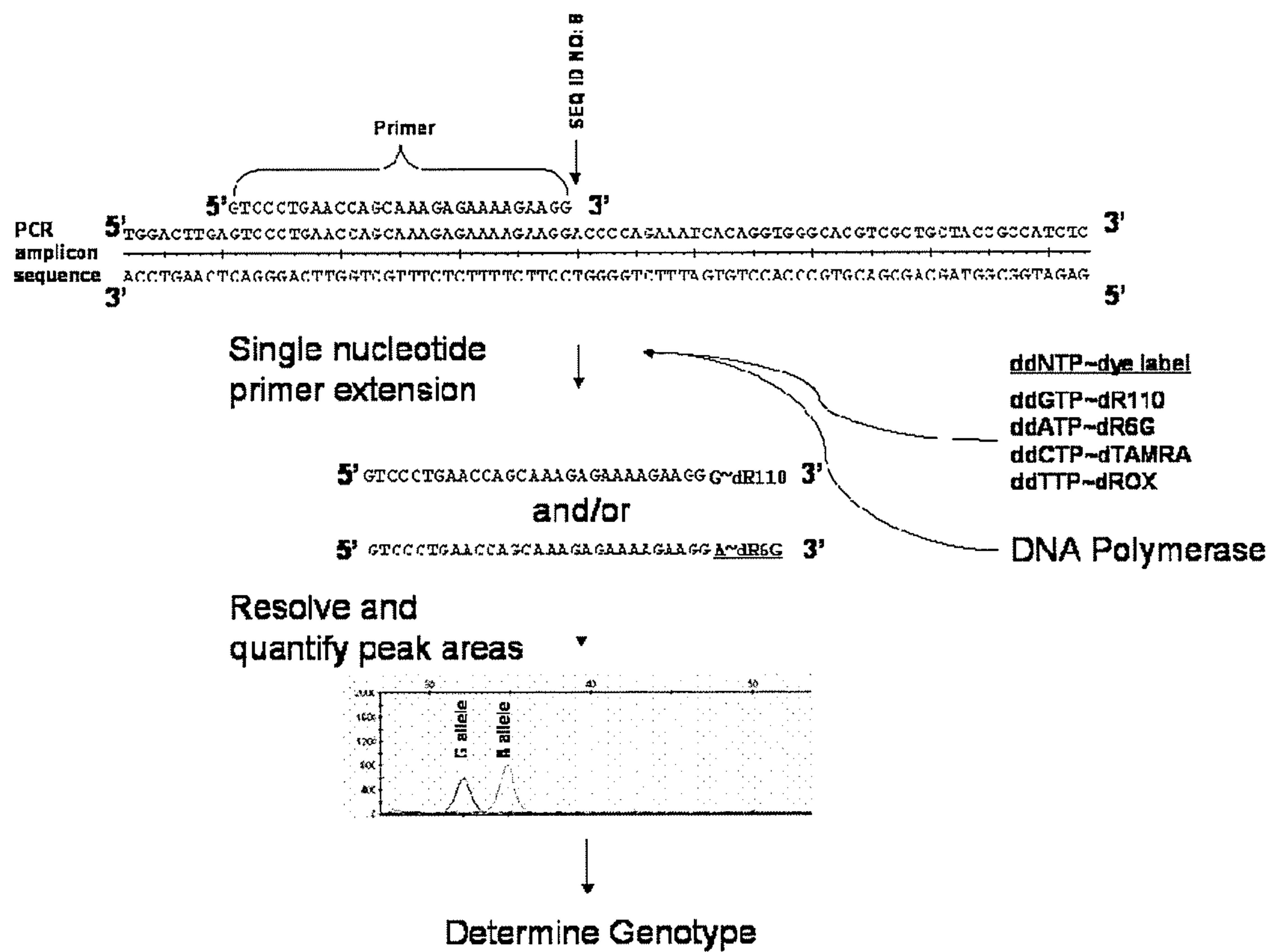
Figure 7. Diagram of Single Nucleotide Primer Extension Assay.
